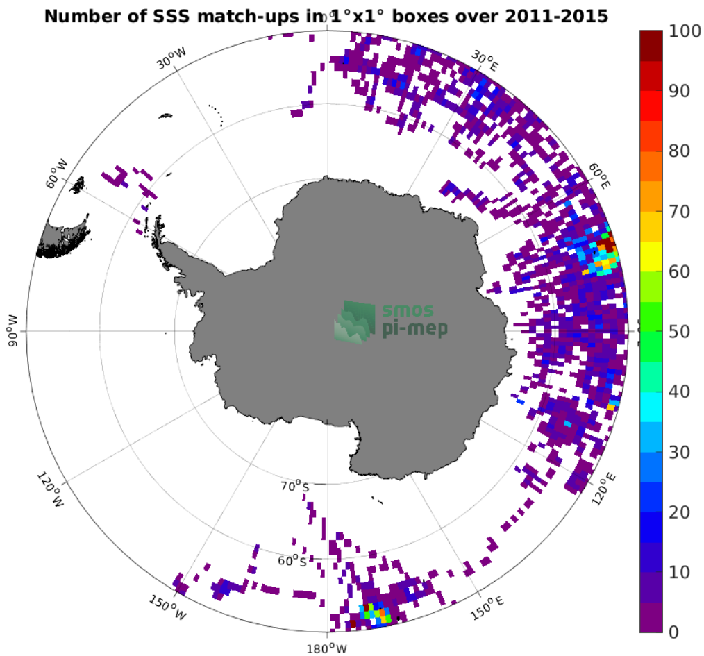
Figure 4: Number of SSS match-ups between Marine mammals SSS and the Aquarius SSS L2 OR v5 (NASA-GSFC) SSS product for the Southern Ocean Pi-MEP region over 1^\circ \times 1^\circ boxes and for the full satellite product period.
