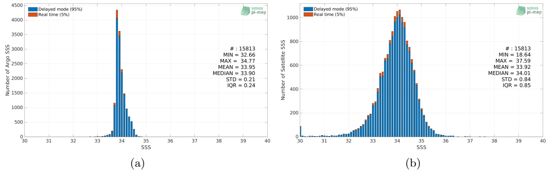
Figure 2: Histograms of SSS from Argo (a) and Aquarius SSS L2 OR v5 (NASA-GSFC) (b) considering all match-up pairs per bins of 0.1 over the Southern Ocean Pi-MEP region and for the full satellite product period.
