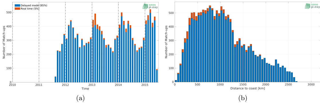
Figure 1: Number of match-ups between Argo and Aquarius SSS L2 OR v5 (NASA-GSFC) SSS as a function of time (a) and as function of the distance to coast (b) over the Southern Ocean Pi-MEP region and for the full satellite product period.
