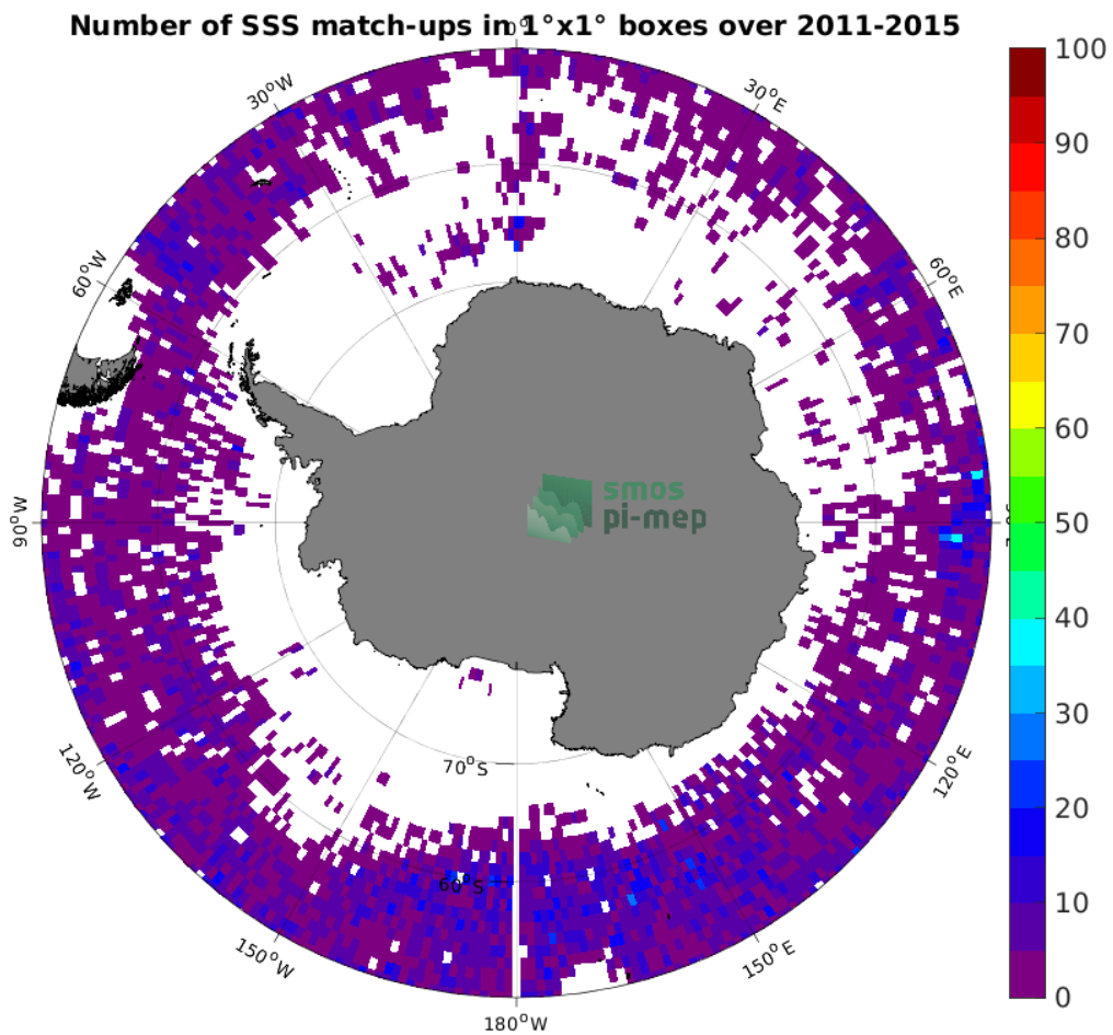
Figure 4: Number of SSS match-ups between Argo SSS and the Aquarius SSS L2 OR v5 (NASA-GSFC) SSS product for the Southern Ocean Pi-MEP region over 1^\circ \times 1^\circ boxes and for the full satellite product period.
