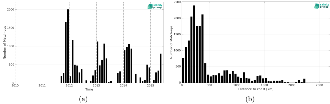
Figure 2: Number of match-ups between TSG (SAMOS) and Aquarius SSS L2 CAP v5 (JPL) SSS as a function of time (a) and as function of the distance to coast (b) over the Southern Ocean Pi-MEP region and for the full satellite product period.
