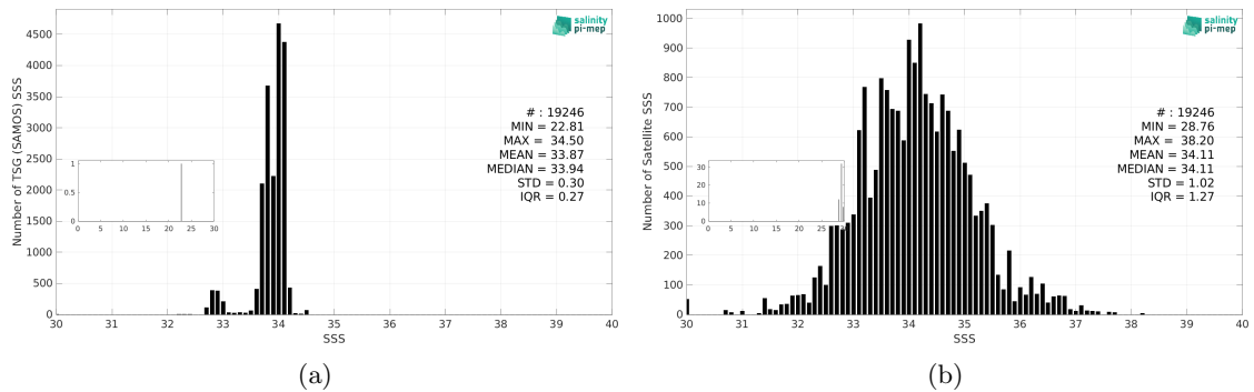
Figure 3: Histograms of SSS from TSG (SAMOS) (a) and Aquarius SSS L2 CAP v5 (JPL) (b) considering all match-up pairs per bins of 0.1 over the Southern Ocean Pi-MEP region and for the full satellite product period.
