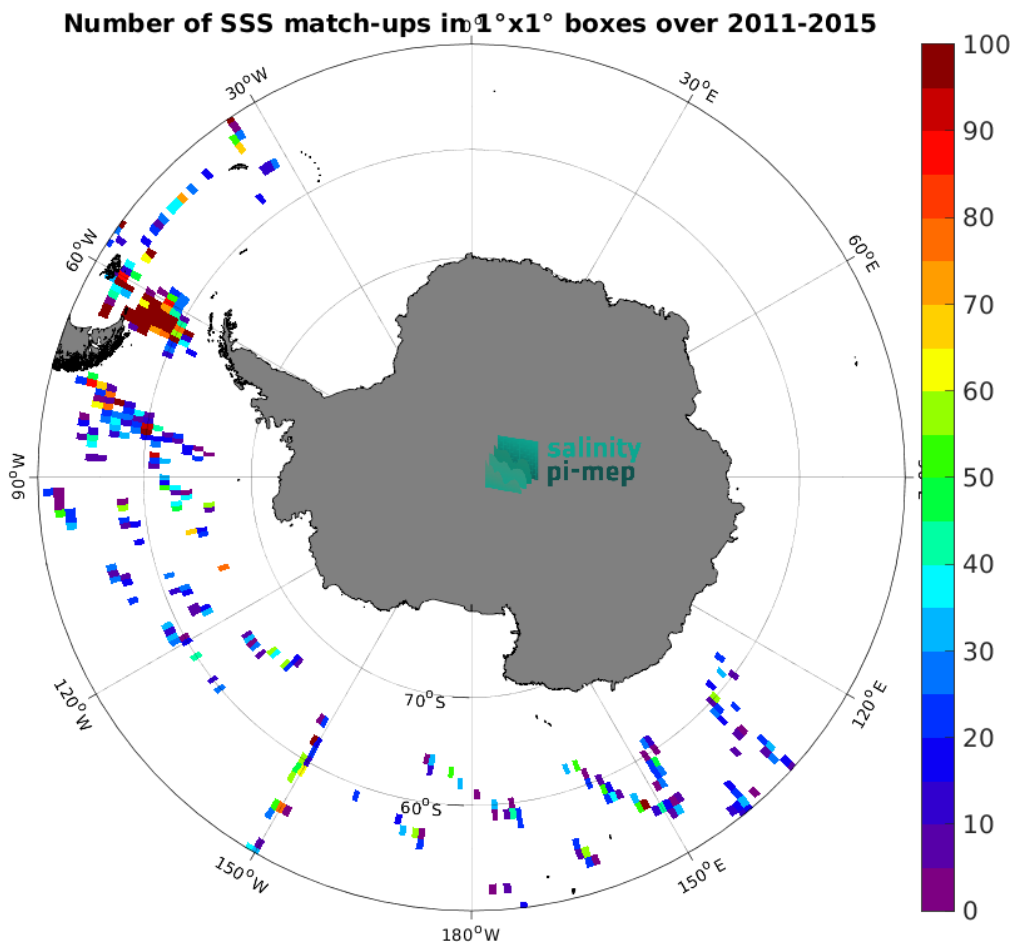
Figure 5: Number of SSS match-ups between TSG (SAMOS) SSS and the Aquarius SSS L2 CAP v5 (JPL) SSS product for the Southern Ocean Pi-MEP region over 1^\circ \times 1^\circ boxes and for the full satellite product period.
