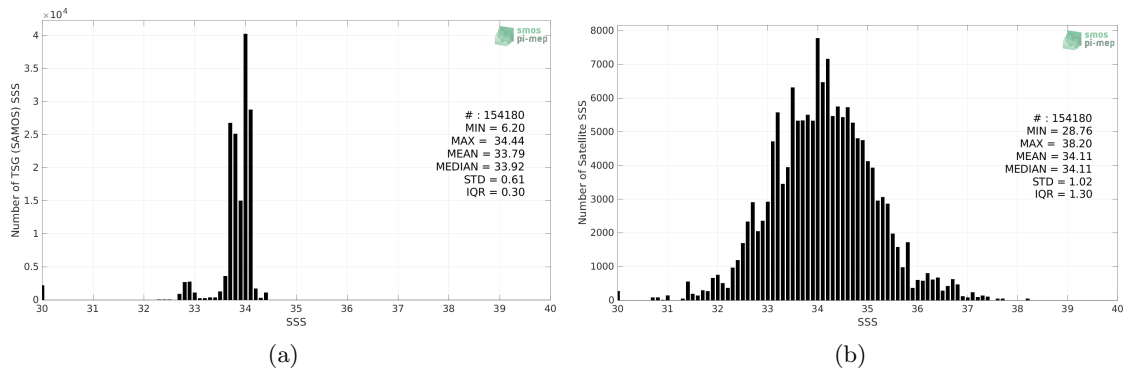
Figure 2: Histograms of SSS from TSG (SAMOS) (a) and Aquarius SSS L2 CAP v5 (JPL) (b) considering all match-up pairs per bins of 0.1 over the Southern Ocean Pi-MEP region and for the full satellite product period.
