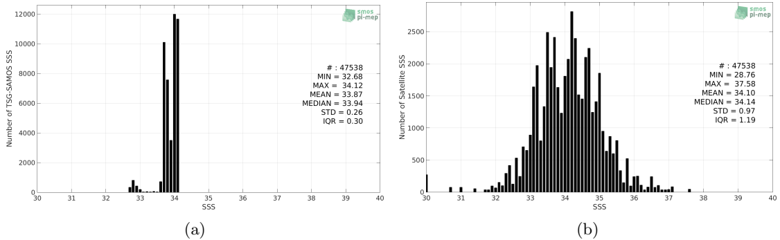
Figure 2: Histograms of SSS from TSG-SAMOS (a) and Aquarius-L2-JPL-V5 (b) considering all match-up pairs per bins of 0.1 over the Southern Ocean Pi-MEP region and for the full satellite product period.
