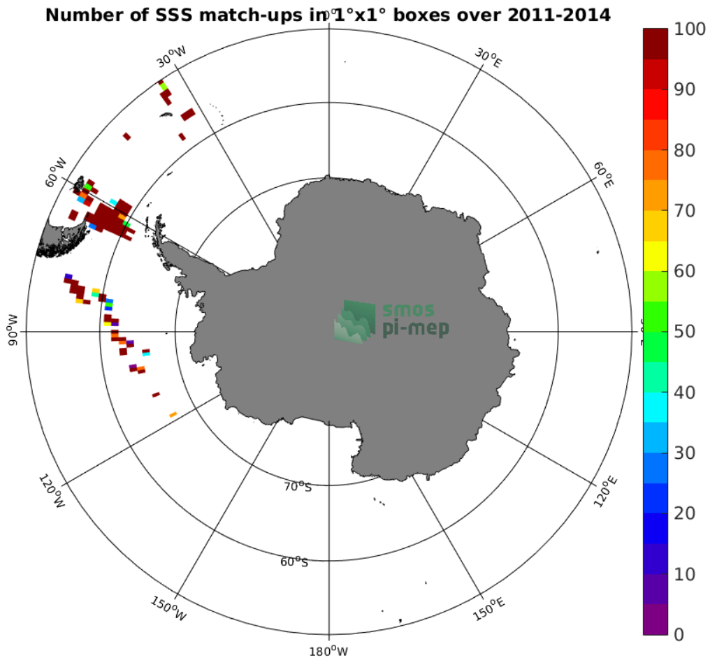
Figure 4: Number of SSS match-ups between TSG-SAMOS SSS and the Aquarius-L2-JPL-V5 SSS product for the Southern Ocean Pi-MEP region over 1°x1° boxes and for the full satellite product period.
