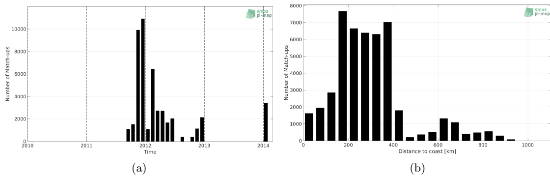
Figure 1: Number of match-ups between TSG-SAMOS and Aquarius-L2-JPL-V5 SSS as a function of time (a) and as function of the distance to coast (b) over the Southern Ocean Pi-MEP region and for the full satellite product period.
