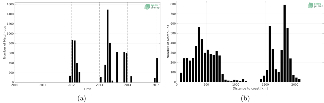
Figure 1: Number of match-ups between TSG (Polarstern) and Aquarius SSS L2 CAP v5 (JPL) SSS as a function of time (a) and as function of the distance to coast (b) over the Southern Ocean Pi-MEP region and for the full satellite product period.
