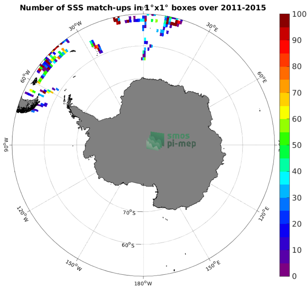
Figure 4: Number of SSS match-ups between TSG (Polarstern) SSS and the Aquarius SSS L2 CAP v5 (JPL) SSS product for the Southern Ocean Pi-MEP region over 1^\circ \times 1^\circ boxes and for the full satellite product period.
