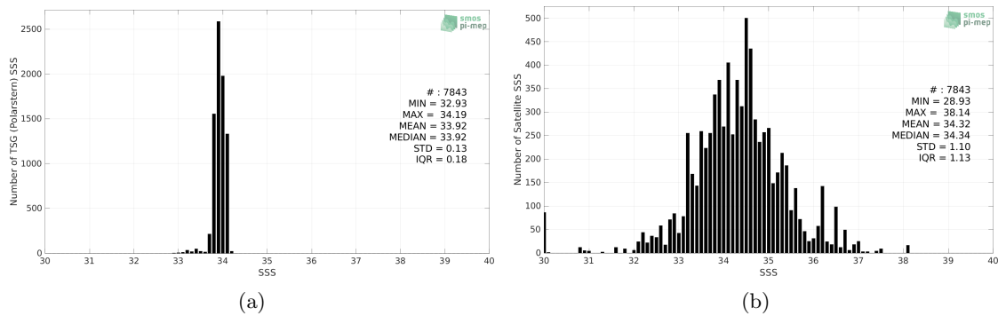
Figure 2: Histograms of SSS from TSG (Polarstern) (a) and Aquarius SSS L2 CAP v5 (JPL) (b) considering all match-up pairs per bins of 0.1 over the Southern Ocean Pi-MEP region and for the full satellite product period.
