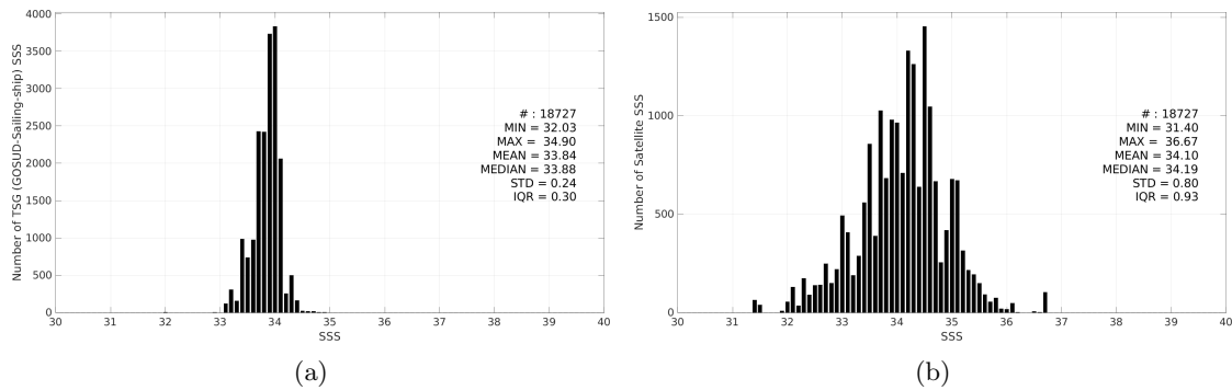
Figure 3: Histograms of SSS from TSG (GOSUD-Sailing-ship) (a) and Aquarius SSS L2 CAP v5 (JPL) (b) considering all match-up pairs per bins of 0.1 over the Southern Ocean Pi-MEP region and for the full satellite product period.
