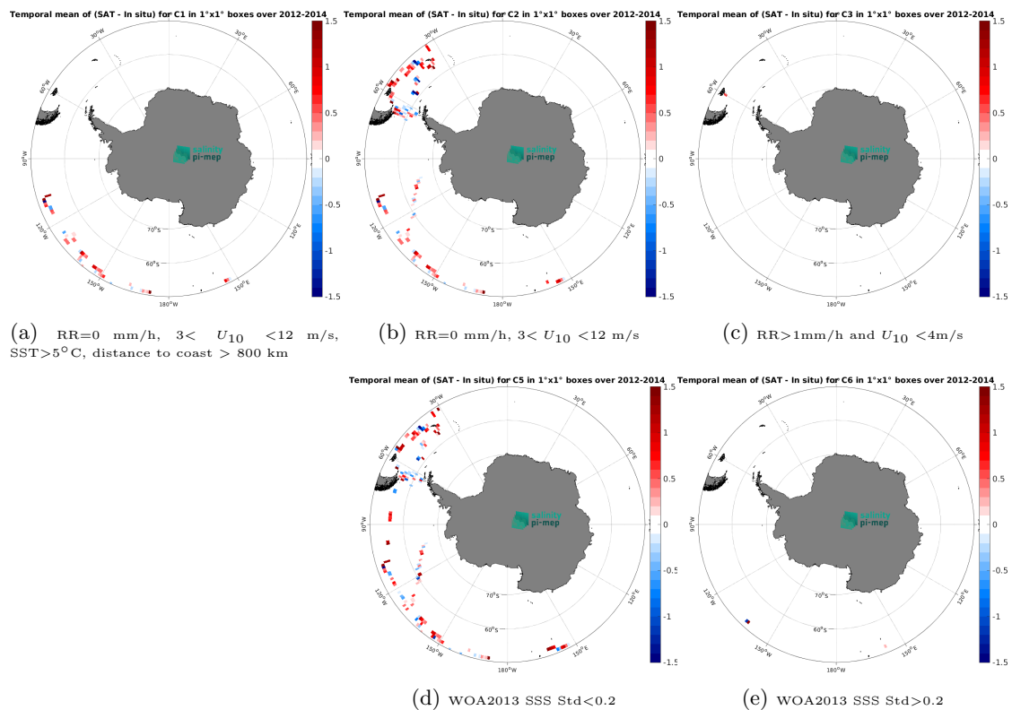
Figure 14: Temporal mean gridded over spatial boxes of size 1^\circ \times 1^\circ of \Delta\text{SSS} (Aquarius SSS L2 CAP v5 (JPL) - TSG (GOSUD-Sailing-ship)) for 5 different subdatasets corresponding to:RR=0 mm/h, 3 < U_{10} < 12 m/s, SST>5°C, distance to coast > 800 km (a), RR=0 mm/h, 3 < U_{10} < 12 m/s (b), RR>1mm/h and U_{10} < 4 m/s (c), WOA2013 SSS Std<0.2 (d), WOA2013 SSS Std>0.2 (e).
