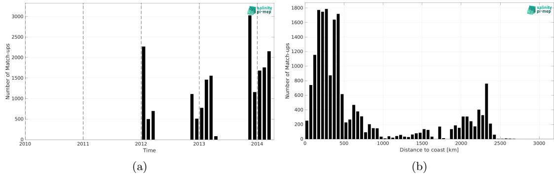
Figure 2: Number of match-ups between TSG (GOSUD-Sailing-ship) and Aquarius SSS L2 CAP v5 (JPL) SSS as a function of time (a) and as function of the distance to coast (b) over the Southern Ocean Pi-MEP region and for the full satellite product period.
