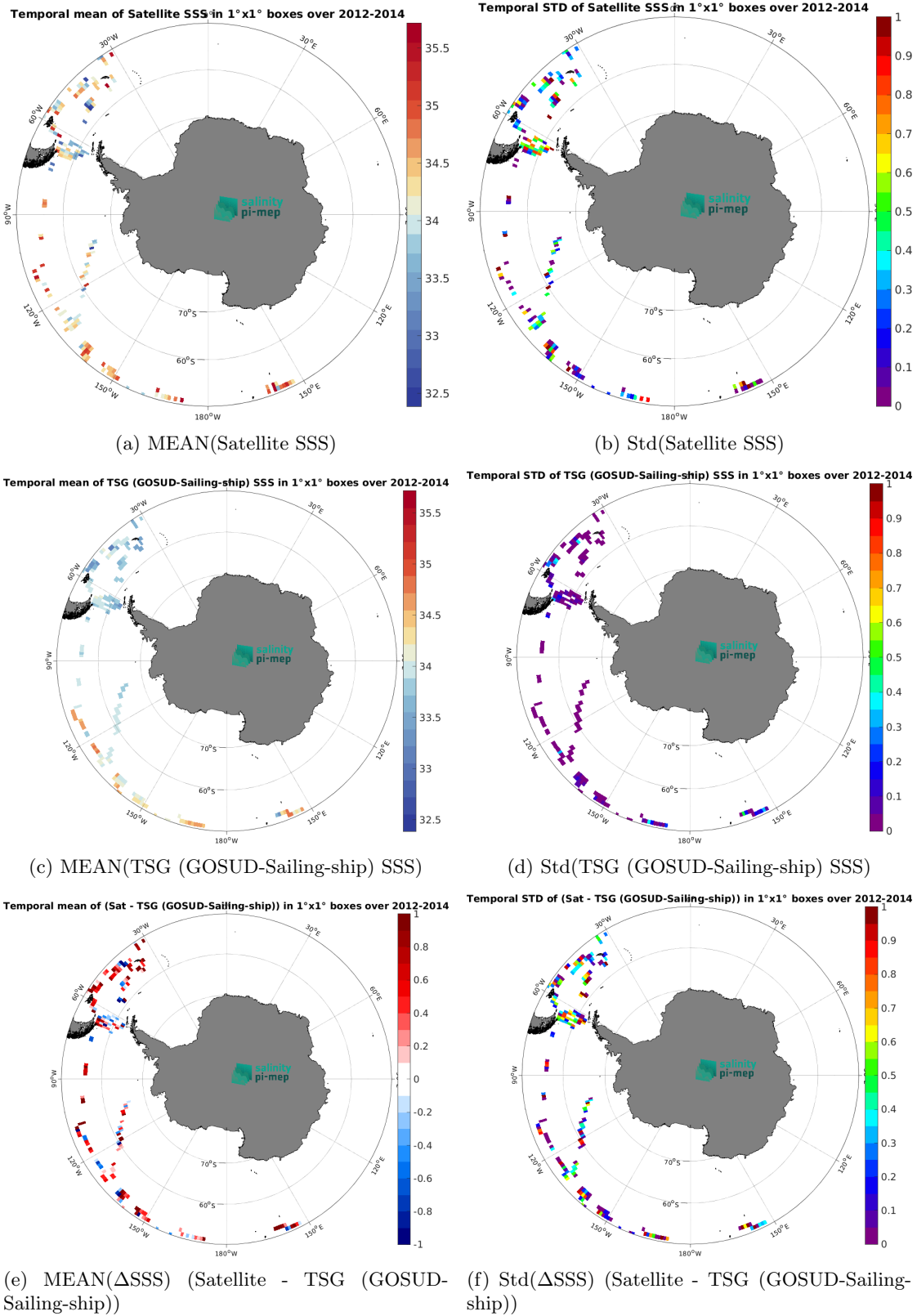
Figure 7: Temporal mean (left) and Std (right), of SSS from Aquarius SSS L2 CAP v5 (JPL) (top), TSG (GOSUD-Sailing-ship) (middle), and of \Delta SSS (Satellite - TSG (GOSUD-Sailing-ship)). Only match-up pairs are used to generate these maps.
