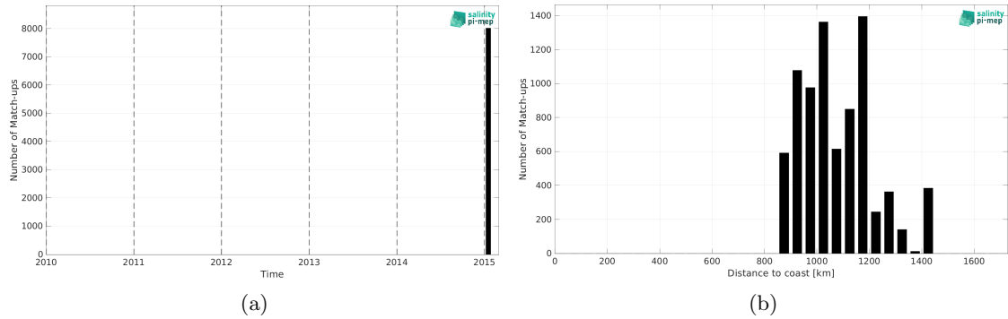
Figure 2: Number of match-ups between TSG (GOSUD-Research-vessel) and Aquarius SSS L2 CAP v5 (JPL) SSS as a function of time (a) and as function of the distance to coast (b) over the Southern Ocean Pi-MEP region and for the full satellite product period.
