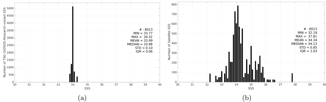
Figure 3: Histograms of SSS from TSG (GOSUD-Research-vessel) (a) and Aquarius SSS L2 CAP v5 (JPL) (b) considering all match-up pairs per bins of 0.1 over the Southern Ocean Pi-MEP region and for the full satellite product period.
