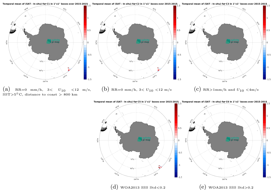
Figure 14: Temporal mean gridded over spatial boxes of size 1^\circ \times 1^\circ of \Delta\text{SSS} (Aquarius SSS L2 CAP v5 (JPL) - TSG (GOSUD-Research-vessel)) for 5 different subdatasets corresponding to:RR=0 mm/h, 3 < U_{10} < 12 m/s, SST > 5^\circ\text{C} , distance to coast > 800 km (a), RR=0 mm/h, 3 < U_{10} < 12 m/s (b), RR > 1 mm/h and U_{10} < 4 m/s (c), WOA2013 SSS Std < 0.2 (d), WOA2013 SSS Std > 0.2 (e).
