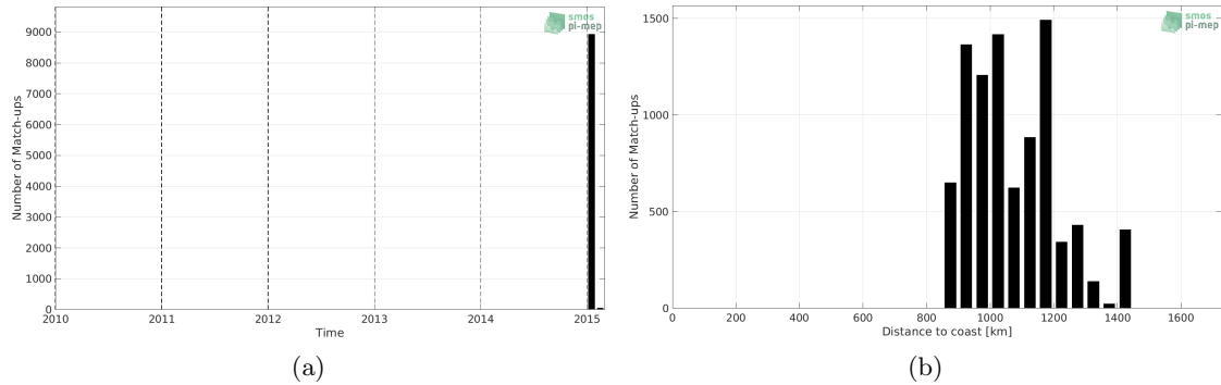
Figure 1: Number of match-ups between TSG (GOSUD-Research-vessel) and Aquarius SSS L2 CAP v5 (JPL) SSS as a function of time (a) and as function of the distance to coast (b) over the Southern Ocean Pi-MEP region and for the full satellite product period.
