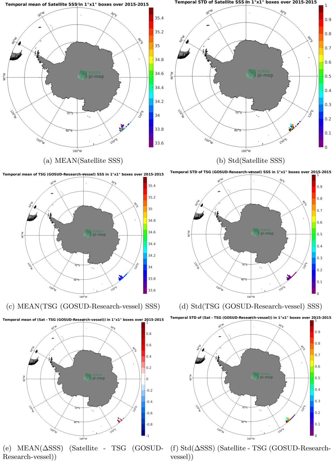
Figure 6: Temporal mean (left) and Std (right) of SSS from Aquarius SSS L2 CAP v5 (JPL) (top), TSG (GOSUD-Research-vessel) (middle), and of \Delta SSS (Satellite - TSG (GOSUD-Research-vessel)). Only match-up pairs are used to generate these maps.
