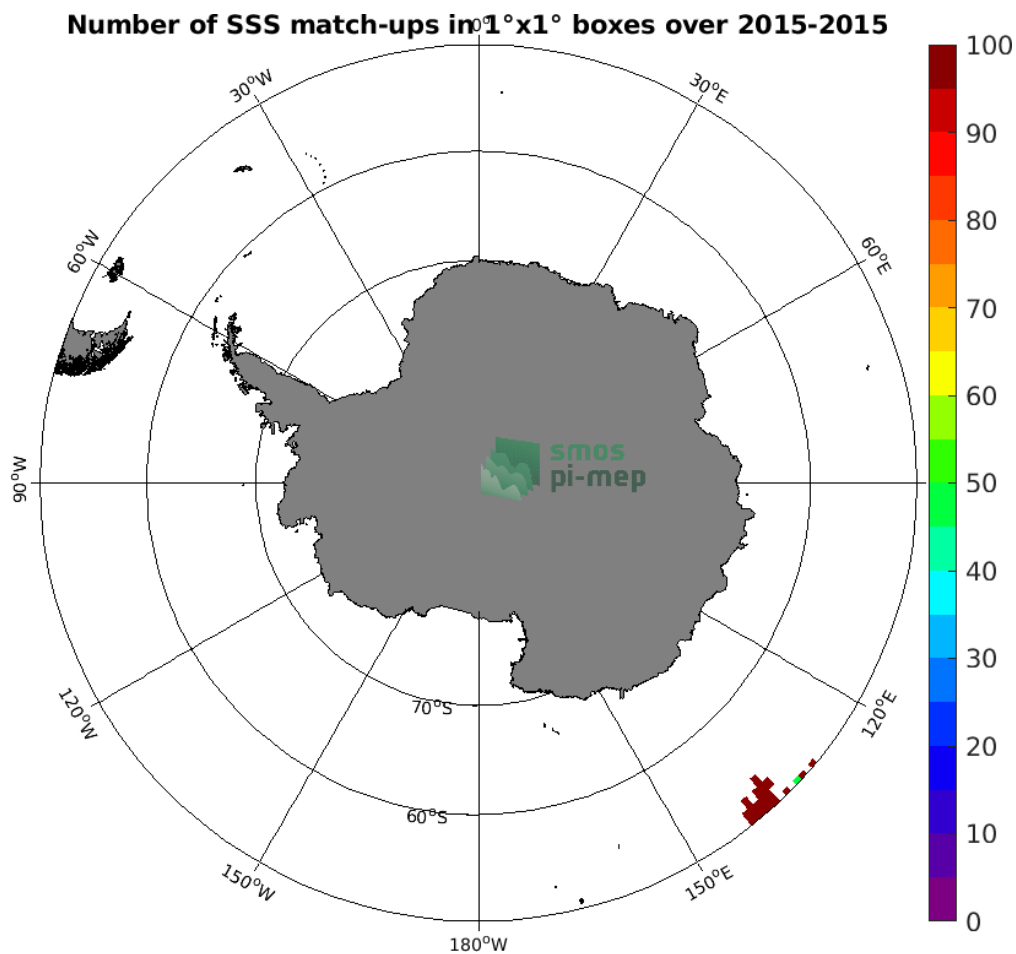
Figure 4: Number of SSS match-ups between TSG (GOSUD-Research-vessel) SSS and the Aquarius SSS L2 CAP v5 (JPL) SSS product for the Southern Ocean Pi-MEP region over 1^\circ \times 1^\circ boxes and for the full satellite product period.
