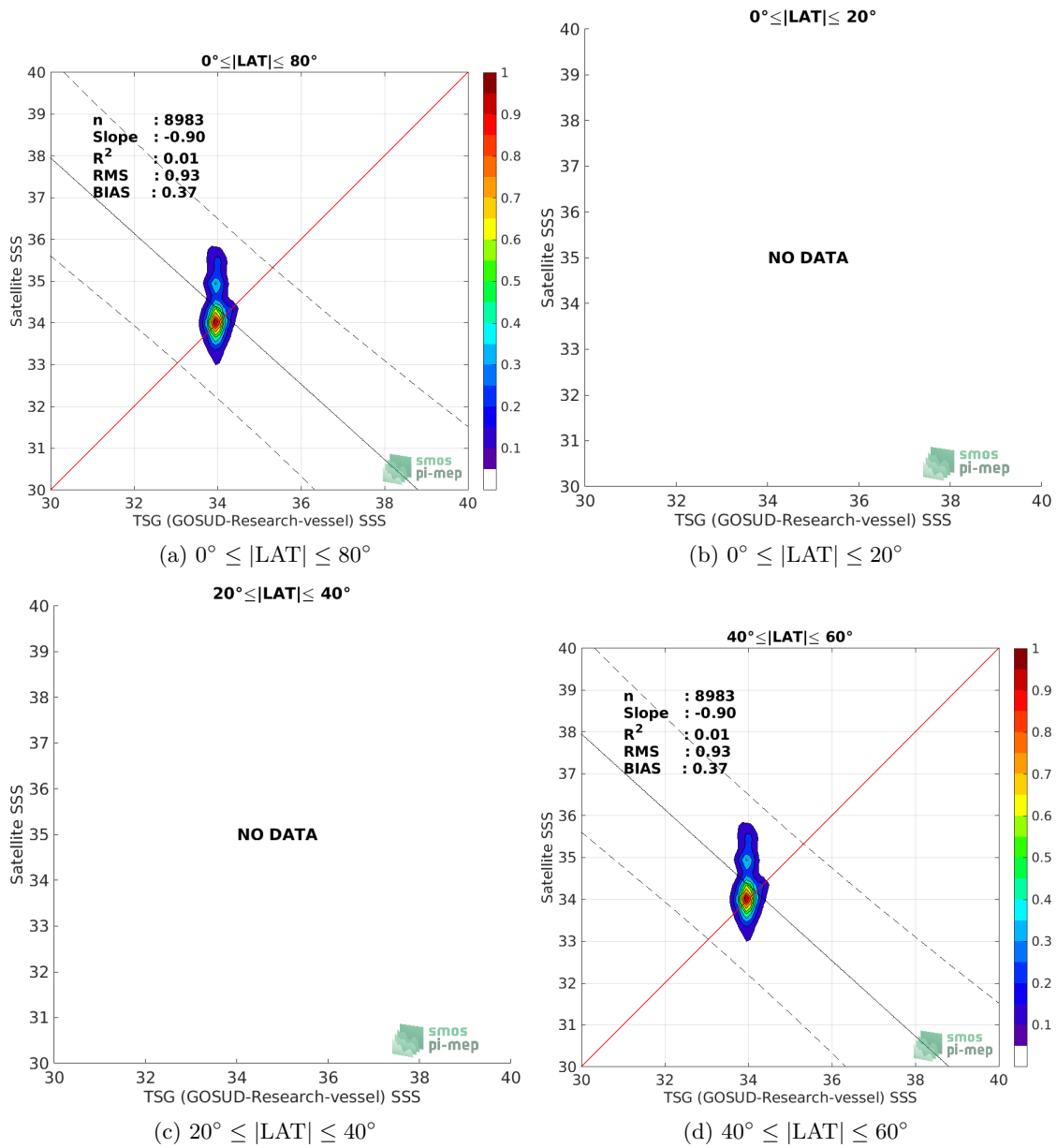
Figure 9: Contour maps of the concentration of Aquarius SSS L2 CAP v5 (JPL) SSS (y-axis) versus TSG (GOSUD-Research-vessel) SSS (x-axis) at match-up pairs for different latitude bands. For each plot, the red line shows x=y . The black thin and dashed lines indicate a linear fit through the data cloud and the \pm 95\% confidence levels, respectively. The number match-up pairs n , the slope and R^2 coefficient of the linear fit, the root mean square (RMS) and the mean bias between satellite and in situ data are indicated for each latitude band in each plots.
