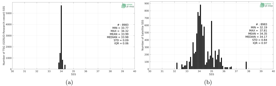
Figure 2: Histograms of SSS from TSG (GOSUD-Research-vessel) (a) and Aquarius SSS L2 CAP v5 (JPL) (b) considering all match-up pairs per bins of 0.1 over the Southern Ocean Pi-MEP region and for the full satellite product period.
