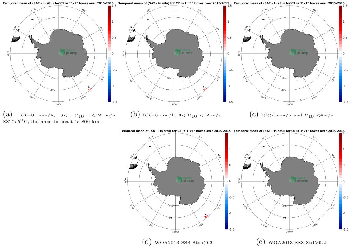
Figure 12: Temporal mean gridded over spatial boxes of size 1^\circ \times 1^\circ of \Delta SSS (Aquarius SSS L2 CAP v5 (JPL) - TSG (GOSUD-Research-vessel)) for 5 different subdatasets corresponding to: RR=0 mm/h, 3 < U_{10} < 12 m/s, SST>5°C, distance to coast > 800 km (a), RR=0 mm/h, 3 < U_{10} < 12 m/s (b), RR>1mm/h and U_{10} < 4 m/s (c), WOA2013 SSS Std<0.2 (d), WOA2013 SSS Std>0.2 (e).
