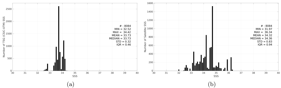
Figure 3: Histograms of SSS from TSG (CSIC-UTM) (a) and Aquarius SSS L2 CAP v5 (JPL) (b) considering all match-up pairs per bins of 0.1 over the Southern Ocean Pi-MEP region and for the full satellite product period.
