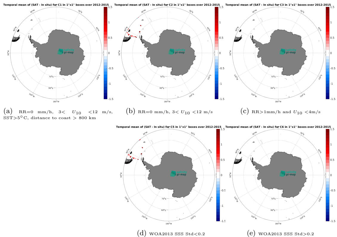
Figure 14: Temporal mean gridded over spatial boxes of size 1^\circ \times 1^\circ of \Delta\text{SSS} (Aquarius SSS L2 CAP v5 (JPL) - TSG (CSIC-UTM)) for 5 different subdatasets corresponding to: RR=0 mm/h, 3 < U_{10} < 12 m/s, SST > 5°C, distance to coast > 800 km (a), RR=0 mm/h, 3 < U_{10} < 12 m/s (b), RR > 1mm/h and U_{10} < 4 m/s (c), WOA2013 SSS Std < 0.2 (d), WOA2013 SSS Std > 0.2 (e).
