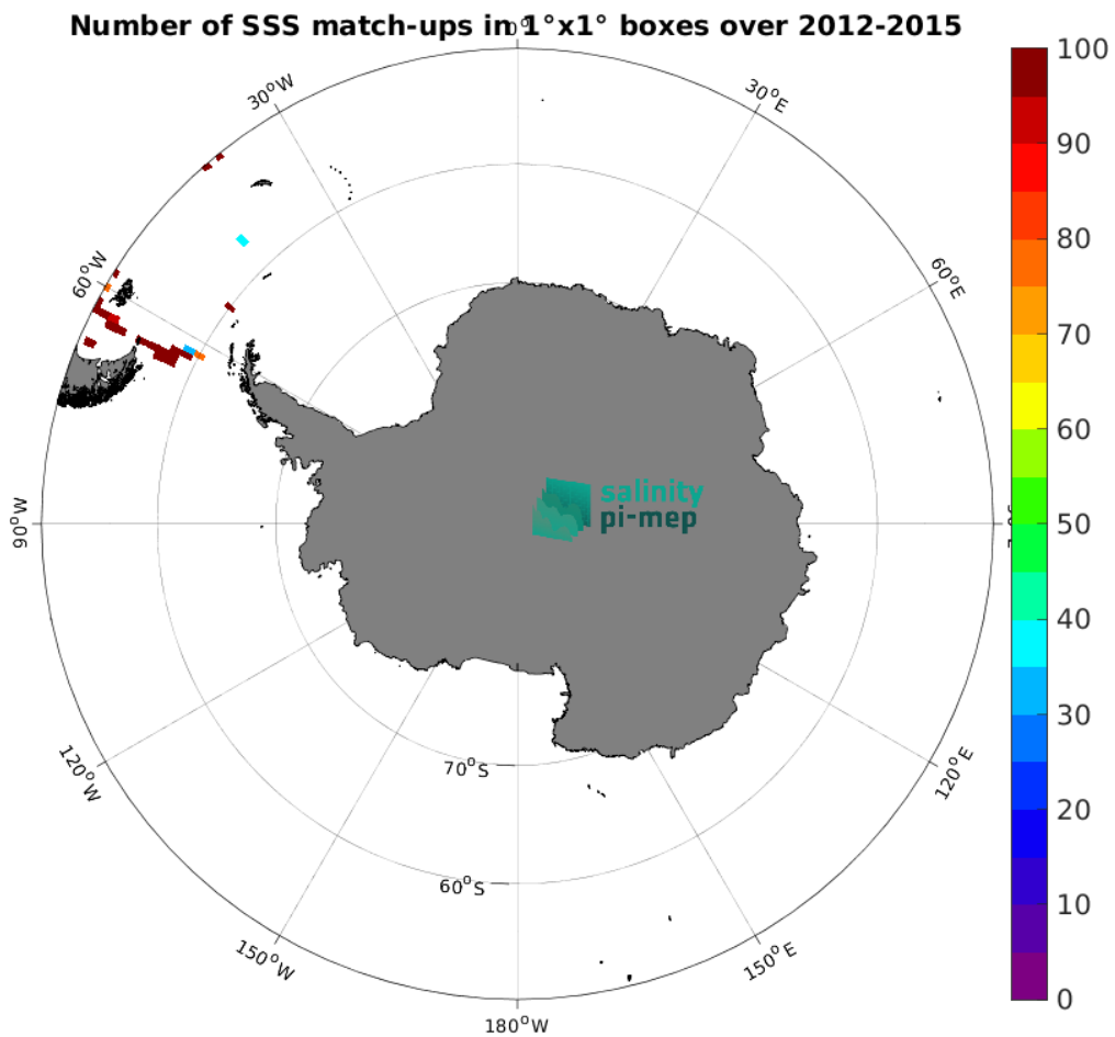
Figure 5: Number of SSS match-ups between TSG (CSIC-UTM) SSS and the Aquarius SSS L2 CAP v5 (JPL) SSS product for the Southern Ocean Pi-MEP region over 1^\circ \times 1^\circ boxes and for the full satellite product period.
