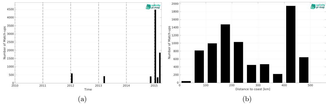
Figure 2: Number of match-ups between TSG (CSIC-UTM) and Aquarius SSS L2 CAP v5 (JPL) SSS as a function of time (a) and as function of the distance to coast (b) over the Southern Ocean Pi-MEP region and for the full satellite product period.
