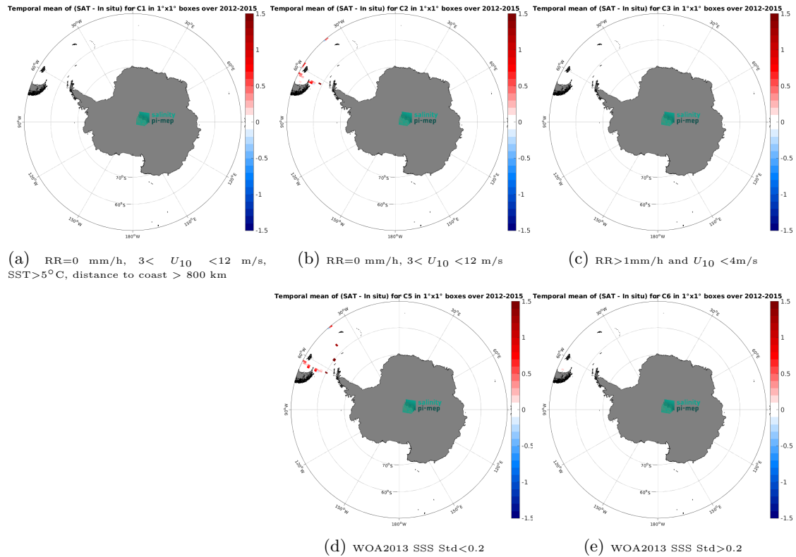
Figure 12: Temporal mean gridded over spatial boxes of size 1^{\circ}\times 1^{\circ} of \Delta\text{SSS} (Aquarius SSS L2 CAP v5 (JPL) - TSG (CSIC-UTM)) for 5 different subdatasets corresponding to: \text{RR}=0 mm/h, 3 < U_{10} < 12 m/s, \text{SST}>5^{\circ}\text{C} , distance to coast > 800 km (a), \text{RR}=0 mm/h, 3 < U_{10} < 12 m/s (b), \text{RR}>1 mm/h and U_{10} < 4 m/s (c), WOA2013 SSS Std < 0.2 (d), WOA2013 SSS Std > 0.2 (e).
