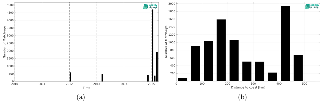
Figure 1: Number of match-ups between TSG (CSIC-UTM) and Aquarius SSS L2 CAP v5 (JPL) SSS as a function of time (a) and as function of the distance to coast (b) over the Southern Ocean Pi-MEP region and for the full satellite product period.
