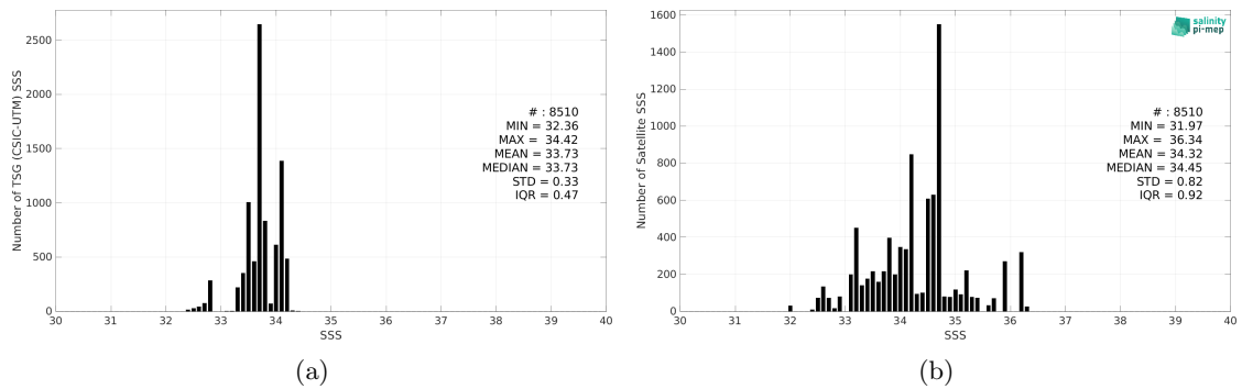
Figure 2: Histograms of SSS from TSG (CSIC-UTM) (a) and Aquarius SSS L2 CAP v5 (JPL) (b) considering all match-up pairs per bins of 0.1 over the Southern Ocean Pi-MEP region and for the full satellite product period.
