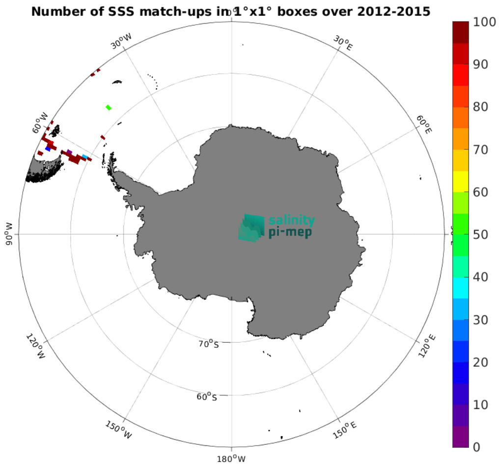
Figure 4: Number of SSS match-ups between TSG (CSIC-UTM) SSS and the Aquarius SSS L2 CAP v5 (JPL) SSS product for the Southern Ocean Pi-MEP region over 1^\circ \times 1^\circ boxes and for the full satellite product period.
