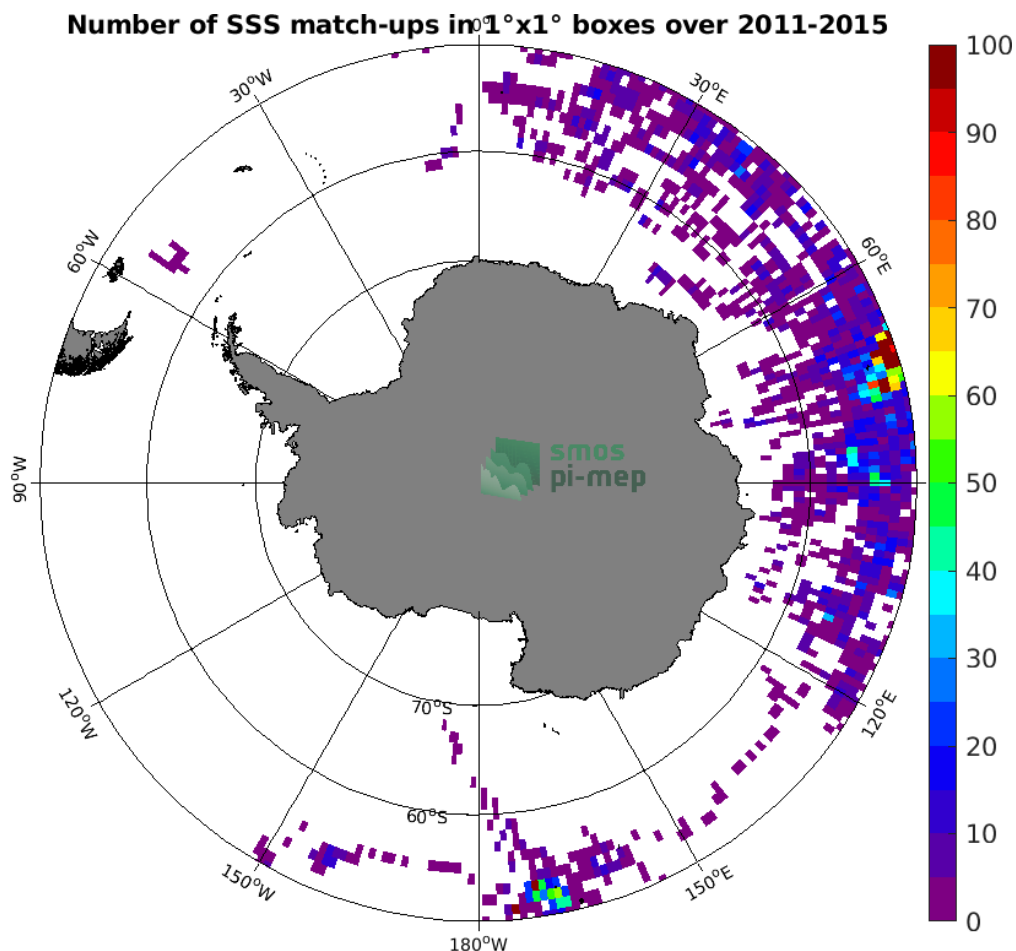
Figure 4: Number of SSS match-ups between Sea mammals SSS and the Aquarius SSS L2 CAP v5 (JPL) SSS product for the Southern Ocean Pi-MEP region over 1^\circ \times 1^\circ boxes and for the full satellite product period.
