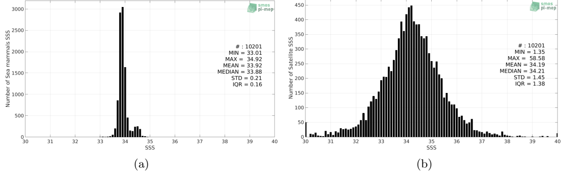
Figure 2: Histograms of SSS from Sea mammals (a) and Aquarius SSS L2 CAP v5 (JPL) (b) considering all match-up pairs per bins of 0.1 over the Southern Ocean Pi-MEP region and for the full satellite product period.
