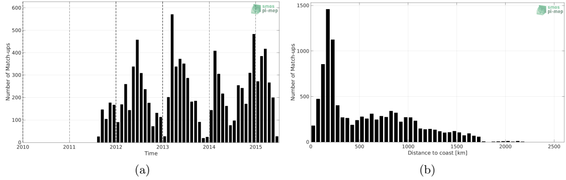
Figure 1: Number of match-ups between Sea mammals and Aquarius SSS L2 CAP v5 (JPL) SSS as a function of time (a) and as function of the distance to coast (b) over the Southern Ocean Pi-MEP region and for the full satellite product period.
