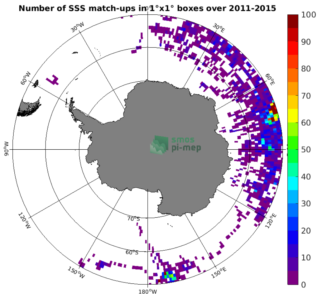
Figure 4: Number of SSS match-ups between Sea mammals SSS and the Aquarius SSS L2 CAP v5 (JPL) SSS product for the Southern Ocean Pi-MEP region over 1^\circ \times 1^\circ boxes and for the full satellite product period.
