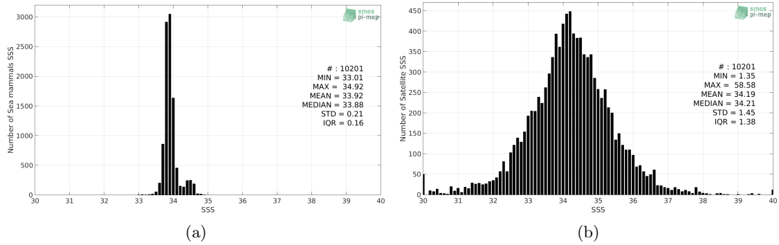
Figure 2: Histograms of SSS from Sea mammals (a) and Aquarius-L2-JPL-V5 (b) considering all match-up pairs per bins of 0.1 over the Southern Ocean Pi-MEP region and for the full satellite product period.
