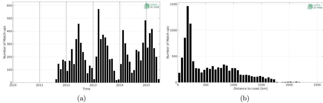
Figure 1: Number of match-ups between Sea mammals and Aquarius-L2-JPL-V5 SSS as a function of time (a) and as function of the distance to coast (b) over the Southern Ocean Pi-MEP region and for the full satellite product period.
