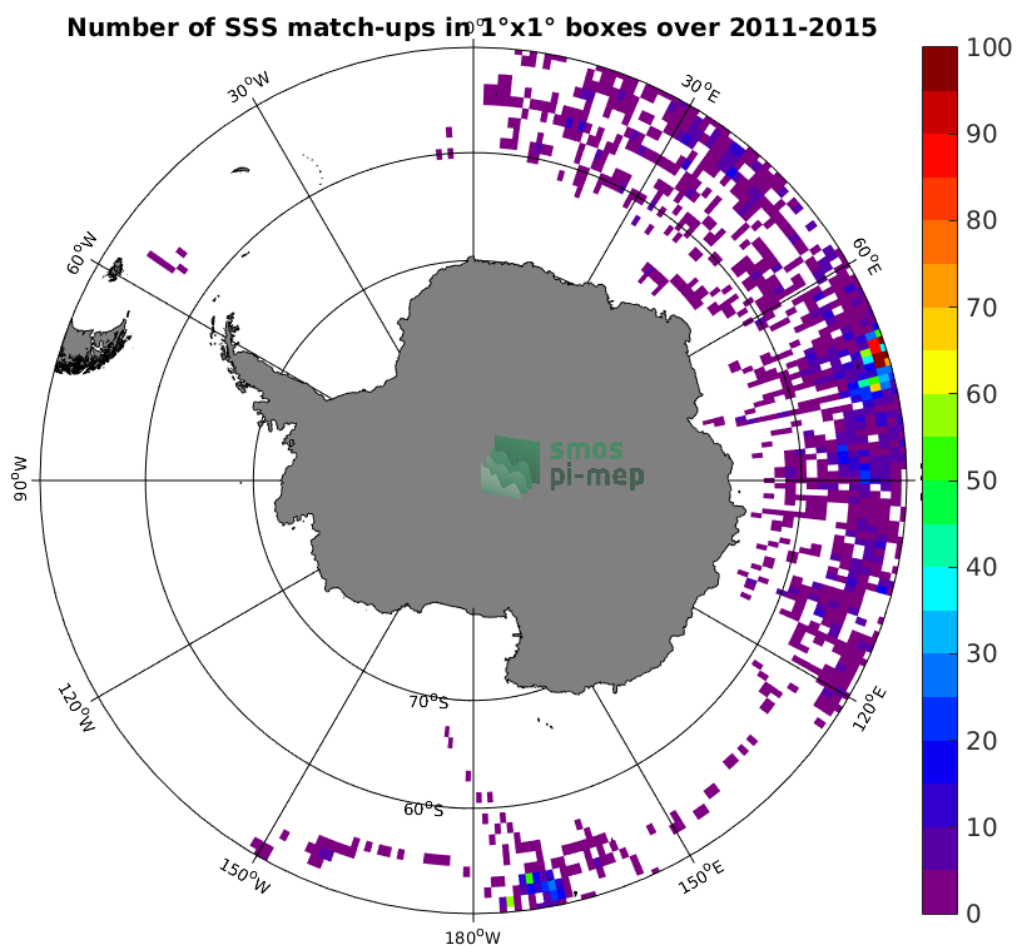
Figure 4: Number of SSS match-ups between Sea mammals SSS and the Aquarius-L2-JPL-V5 SSS product for the Southern Ocean Pi-MEP region over 1^\circ \times 1^\circ boxes and for the full satellite product period.
