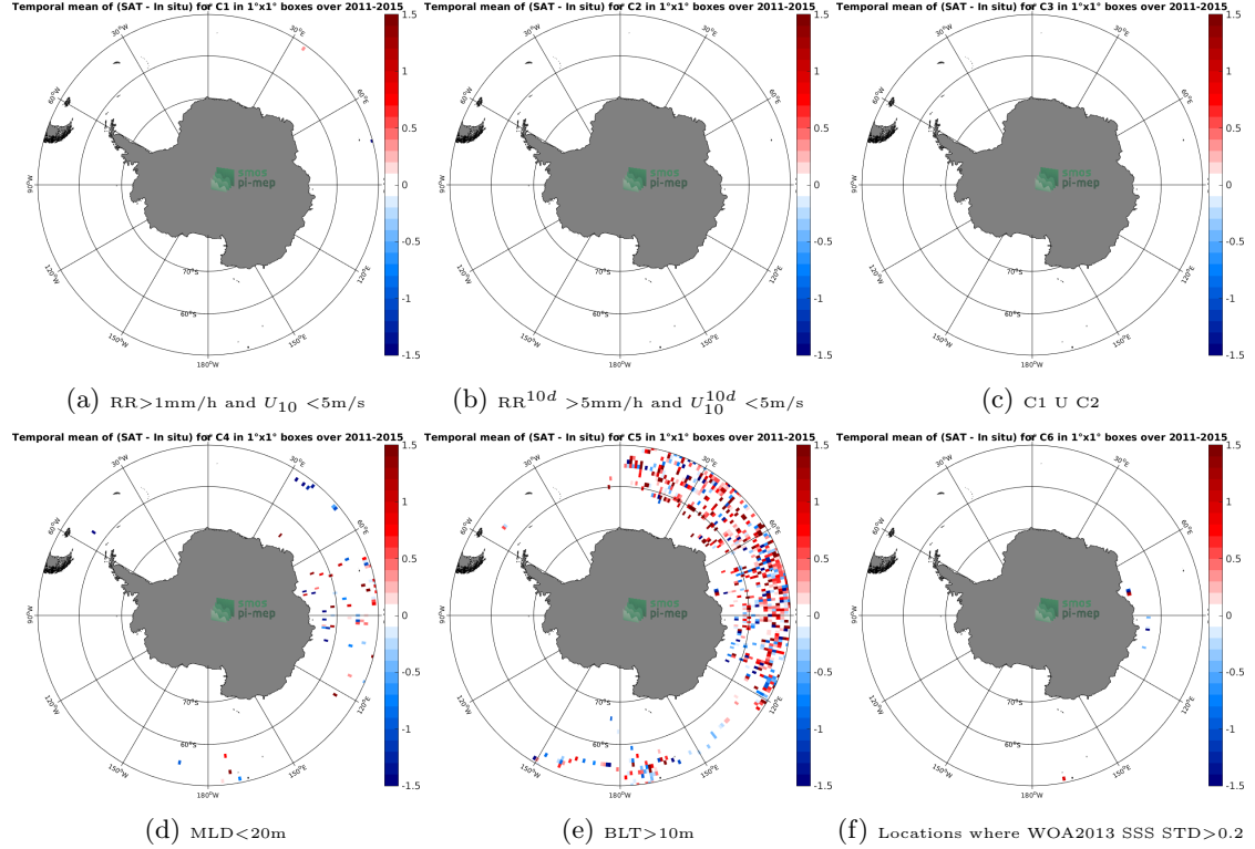
Figure 12: Temporal mean gridded over spatial boxes of size 1^\circ \times 1^\circ of \Delta\text{SSS} (Aquarius-L2-JPL-V5 - Sea mammals) for 6 different subdatasets corresponding to: \text{RR} > 1\text{mm/h} and U_{10} < 5\text{m/s} (a), \text{RR}^{10d} > 5\text{mm/h} and U_{10}^{10d} < 5\text{m/s} (b), C1 U C2 (c), \text{MLD} < 20\text{m} (d), \text{BLT} > 10\text{m} (e), Locations where WOA2013 SSS STD > 0.2 (f).
