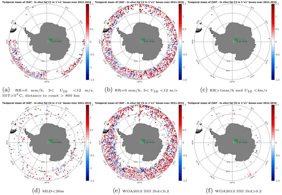
Figure 12: Temporal mean gridded over spatial boxes of size 1^{\circ}\times 1^{\circ} of \Delta\text{SSS} (Aquarius SSS L2 CAP v5 (JPL) - Argo) for 6 different subdatasets corresponding to: \text{RR}=0 mm/h, 3 < U_{10} < 12 m/s, \text{SST}>5^{\circ}\text{C} , distance to coast > 800 km (a), \text{RR}=0 mm/h, 3 < U_{10} < 12 m/s (b), \text{RR}>1\text{mm/h} and U_{10} < 4\text{m/s} (c), \text{MLD}<20\text{m} (d), \text{WOA2013 SSS Std}<0.2 (e), \text{WOA2013 SSS Std}>0.2 (f).
