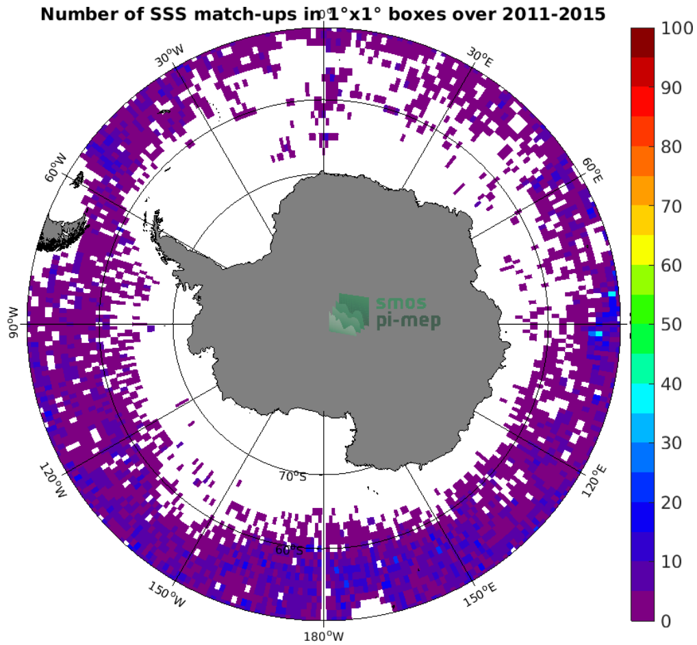
Figure 4: Number of SSS match-ups between Argo SSS and the Aquarius SSS L2 CAP v5 (JPL) SSS product for the Southern Ocean Pi-MEP region over 1^\circ \times 1^\circ boxes and for the full satellite product period.
