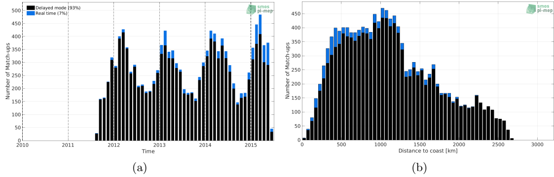
Figure 1: Number of match-ups between Argo and Aquarius SSS L2 CAP v5 (JPL) SSS as a function of time (a) and as function of the distance to coast (b) over the Southern Ocean Pi-MEP region and for the full satellite product period.
