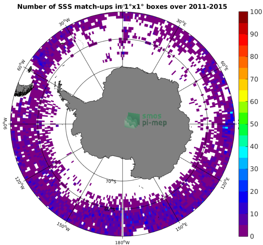
Figure 4: Number of SSS match-ups between Argo SSS and the Aquarius-L2-JPL-V5 SSS product for the Southern Ocean Pi-MEP region over 1^\circ \times 1^\circ boxes and for the full satellite product period.
