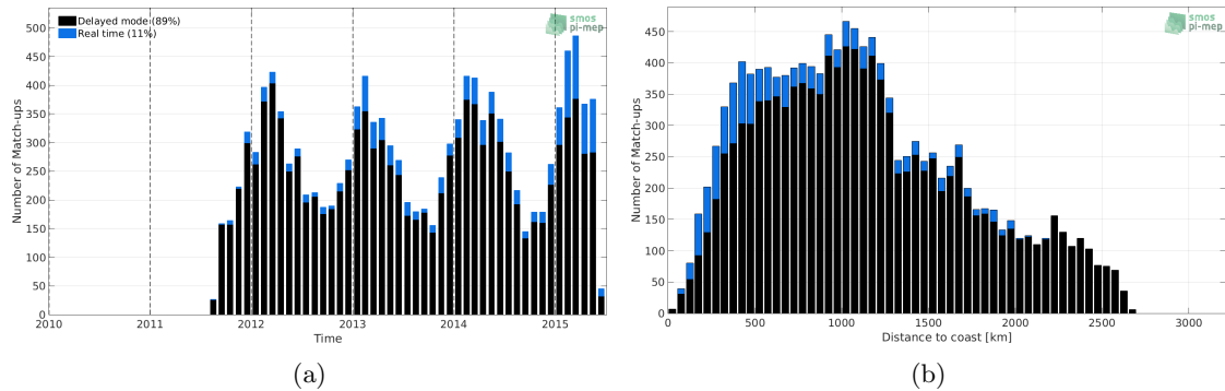
Figure 1: Number of match-ups between Argo and Aquarius-L2-JPL-V5 SSS as a function of time (a) and as function of the distance to coast (b) over the Southern Ocean Pi-MEP region and for the full satellite product period.
