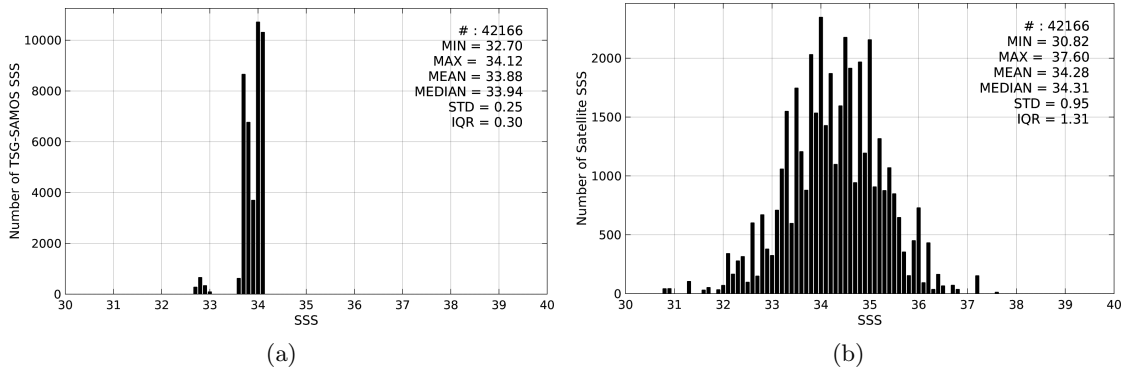
Figure 2: Histograms of SSS from TSG-SAMOS (a) and AQUARIUS-L2-JPL-V4 (b) considering all match-up pairs per bins of 0.1 over the Southern Ocean Pi-MEP region and for the full satellite product period.
