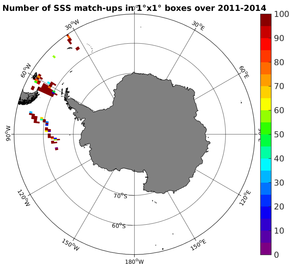
Figure 4: Number of SSS match-ups between TSG-SAMOS SSS and the AQUARIUS-L2-JPL-V4 SSS product for the Southern Ocean Pi-MEP region over 1^\circ \times 1^\circ boxes and for the full satellite product period.
