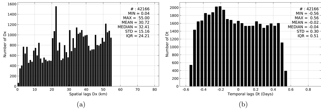
Figure 5: Histograms of the spatial (a) and temporal (b) lags between the time of the TSG-SAMOS measurements and the date of the corresponding AQUARIUS-L2-JPL-V4 SSS product.
