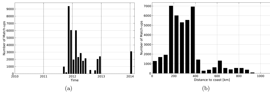
Figure 1: Number of match-ups between TSG-SAMOS and AQUARIUS-L2-JPL-V4 SSS as a function of time (a) and as function of the distance to coast (b) over the Southern Ocean Pi-MEP region and for the full satellite product period.
