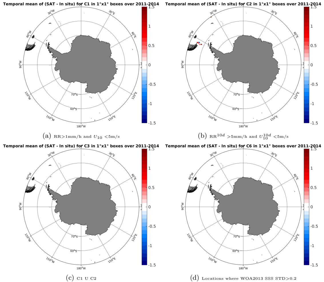
Figure 12: Temporal mean gridded over spatial boxes of size 1°x1° of \Delta SSS (AQUARIUS-L2-JPL-V4 - TSG-SAMOS) for 4 different subdatasets corresponding to: RR > 1\text{mm/h} and U_{10} < 5\text{m/s} (a), RR^{10d} > 5\text{mm/h} and U_{10}^{10d} < 5\text{m/s} (b), C1 U C2 (c), Locations where WOA2013 SSS STD > 0.2 (d).
