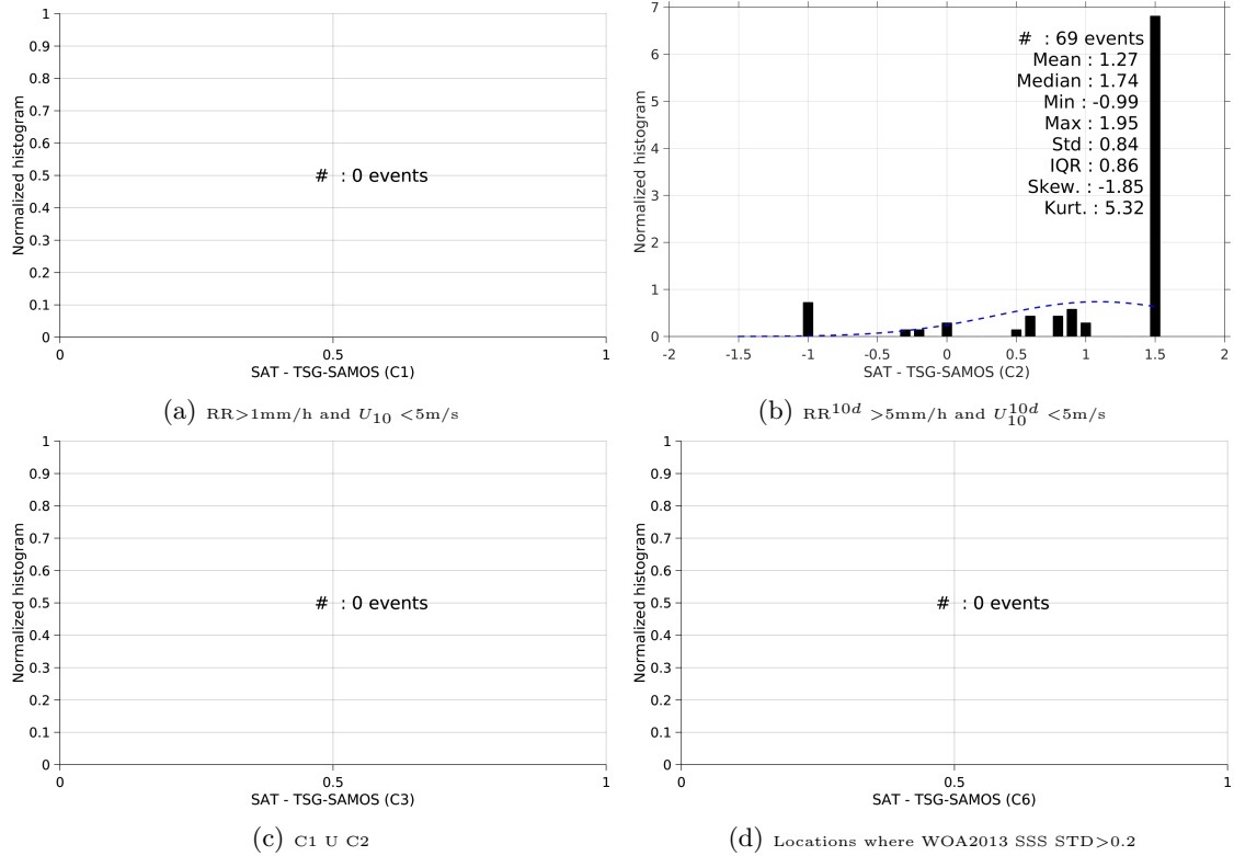
Figure 13: Normalized histogram of \Delta\text{SSS} (AQUARIUS-L2-JPL-V4 - TSG-SAMOS) for 6 different subdatasets corresponding to: RR > 1\text{mm/h} and U_{10} < 5\text{m/s} (a), RR^{10d} > 5\text{mm/h} and U_{10}^{10d} < 5\text{m/s} (b), C1 U C2 (c), Locations where WOA2013 SSS STD > 0.2 (d).
