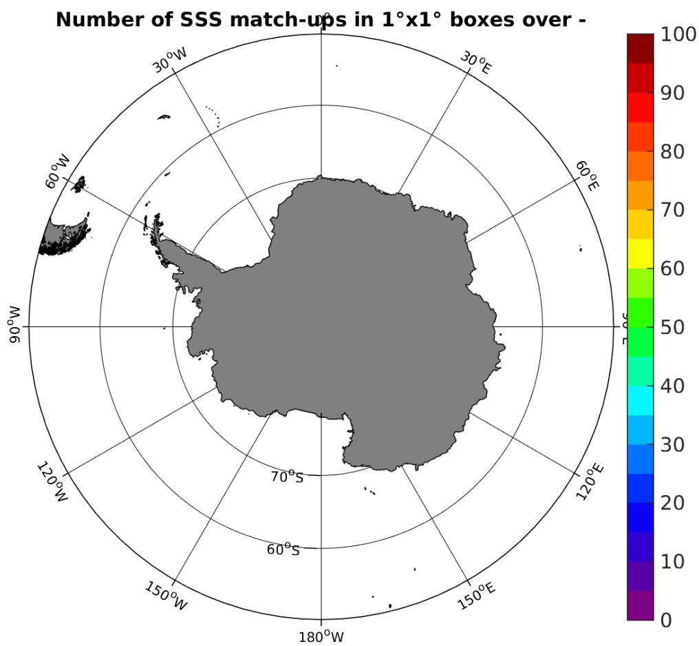
Figure 4: Number of SSS match-ups between TSG-LEGOS-DM SSS and the AQUARIUS-L2-JPL-V4 SSS product for the Southern Ocean Pi-MEP region over 1°x1° boxes and for the full satellite product period.
