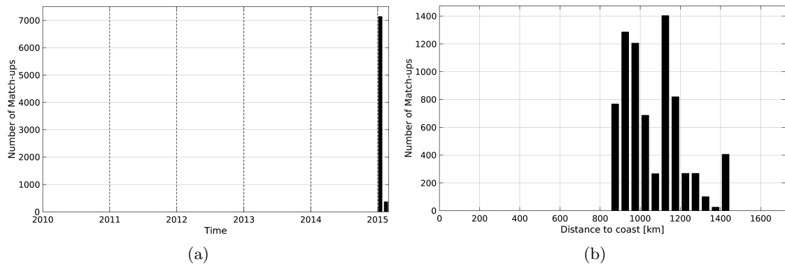
Figure 1: Number of match-ups between TSG-GOSUD-Research-vessel and AQUARIUS-L2-JPL-V4 SSS as a function of time (a) and as function of the distance to coast (b) over the Southern Ocean Pi-MEP region and for the full satellite product period.
