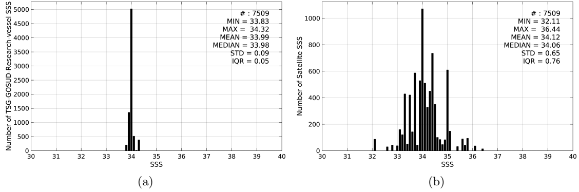
Figure 2: Histograms of SSS from TSG-GOSUD-Research-vessel (a) and AQUARIUS-L2-JPL-V4 (b) considering all match-up pairs per bins of 0.1 over the Southern Ocean Pi-MEP region and for the full satellite product period.
