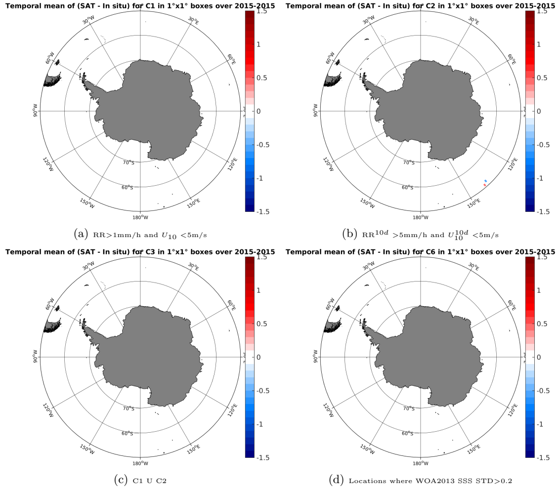
Figure 12: Temporal mean gridded over spatial boxes of size 1^\circ \times 1^\circ of \Delta SSS (AQUARIUS-L2-JPL-V4 - TSG-GOSUD-Research-vessel) for 4 different subdatasets corresponding to: RR > 1mm/h and U_{10} < 5 m/s (a), RR 10d > 5mm/h and U_{10}^{10d} < 5 m/s (b), C1 U C2 (c), Locations where WOA2013 SSS STD > 0.2 (d).
