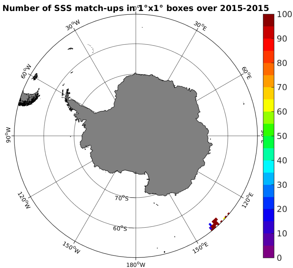
Figure 4: Number of SSS match-ups between TSG-GOSUD-Research-vessel SSS and the AQUARIUS-L2-JPL-V4 SSS product for the Southern Ocean Pi-MEP region over 1^\circ \times 1^\circ boxes and for the full satellite product period.
