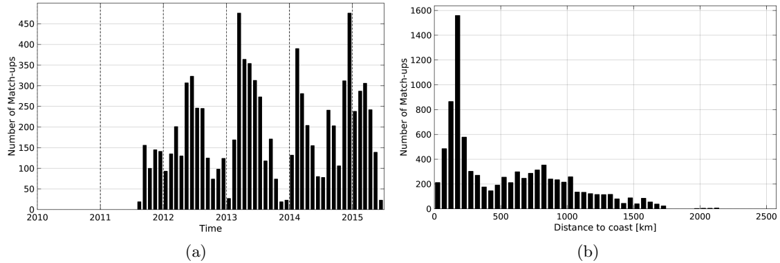
Figure 1: Number of match-ups between Sea mammals and AQUARIUS-L2-JPL-V4 SSS as a function of time (a) and as function of the distance to coast (b) over the Southern Ocean Pi-MEP region and for the full satellite product period.
