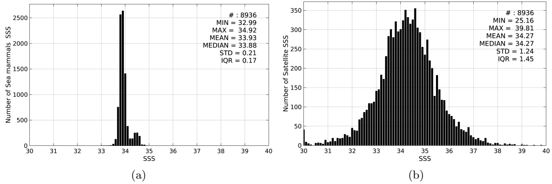
Figure 2: Histograms of SSS from Sea mammals (a) and AQUARIUS-L2-JPL-V4 (b) considering all match-up pairs per bins of 0.1 over the Southern Ocean Pi-MEP region and for the full satellite product period.
