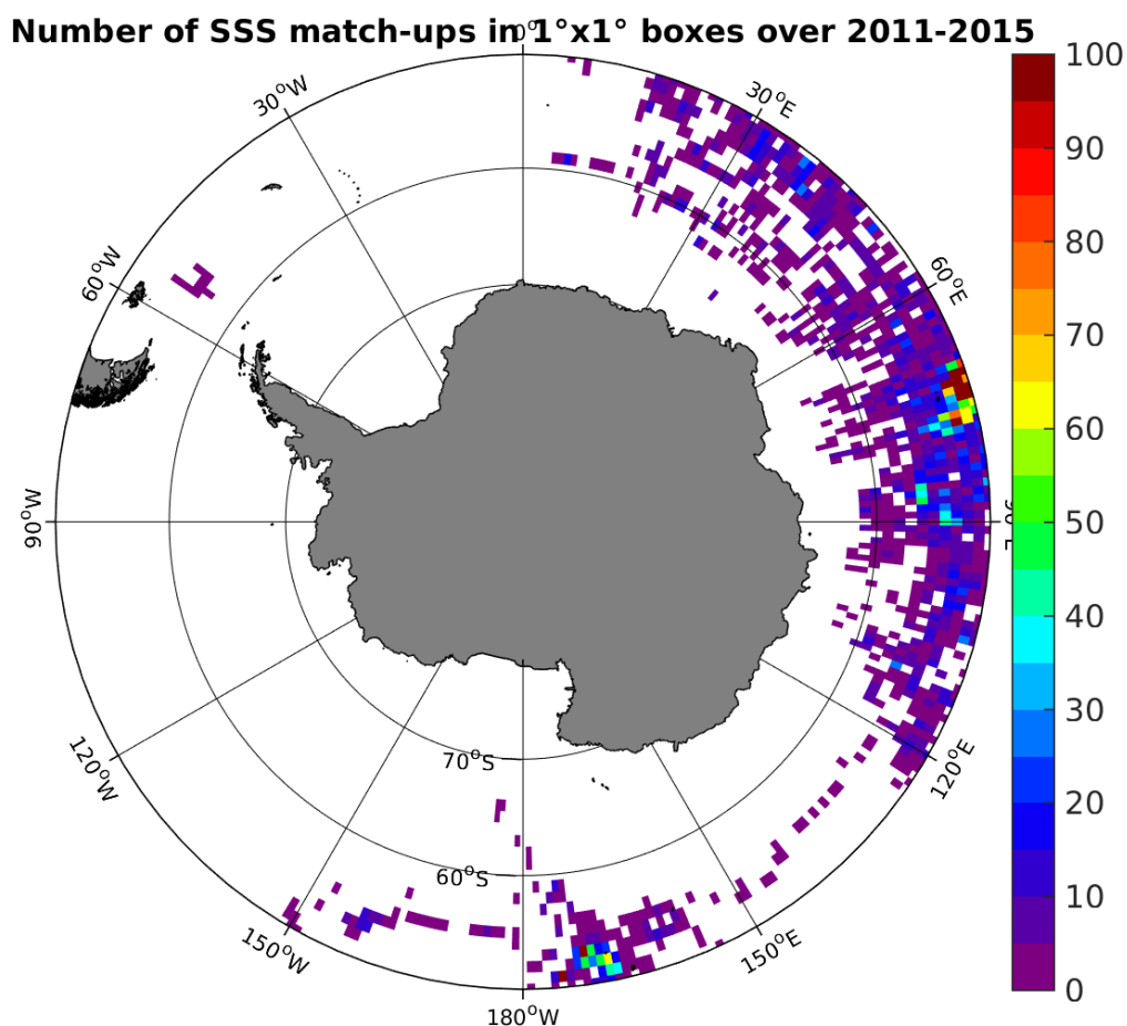
Figure 4: Number of SSS match-ups between Sea mammals SSS and the AQUARIUS-L2-JPL-V4 SSS product for the Southern Ocean Pi-MEP region over 1^\circ \times 1^\circ boxes and for the full satellite product period.
