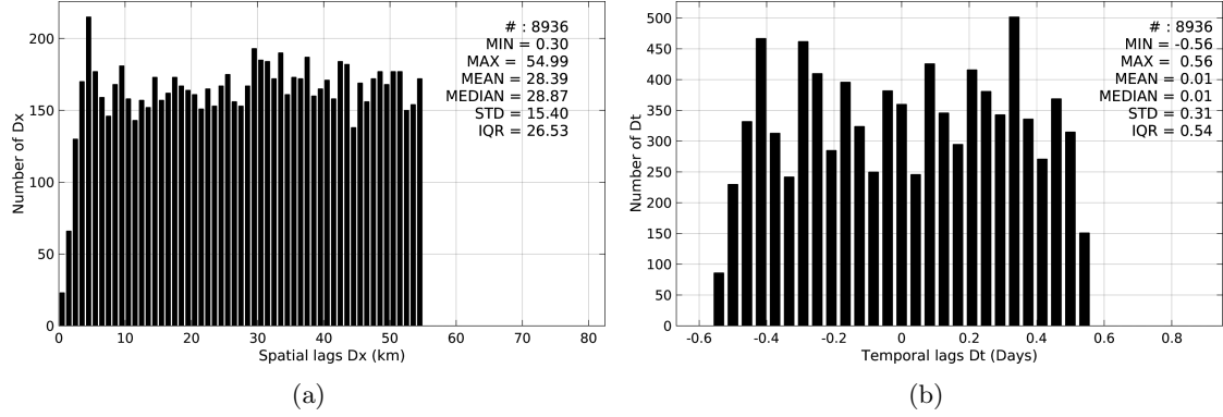
Figure 5: Histograms of the spatial (a) and temporal (b) lags between the time of the Sea mammals measurements and the date of the corresponding AQUARIUS-L2-JPL-V4 SSS product.
