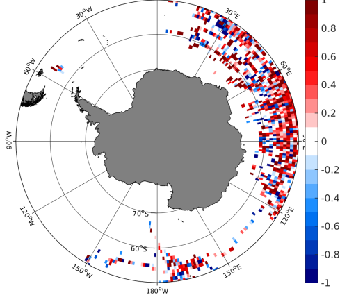
(e) MEAN( \Delta SSS) (Satellite - Sea mammals)
