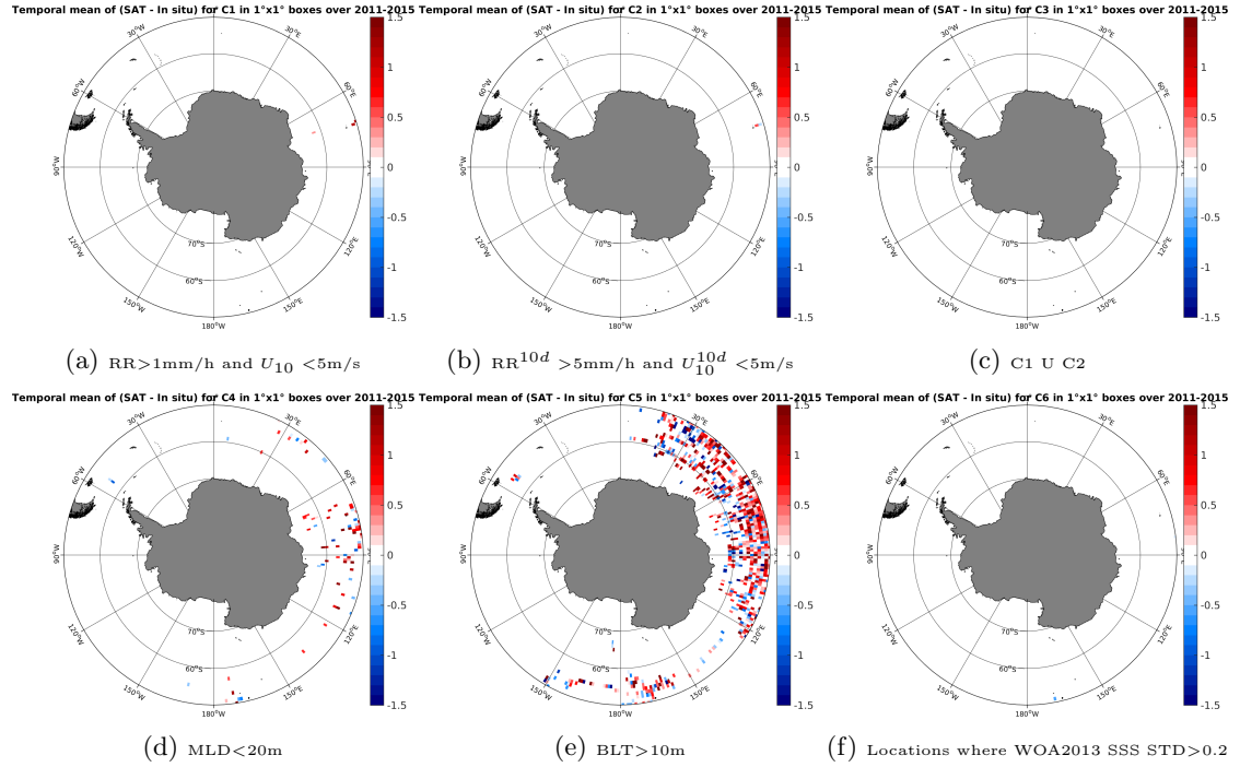
Figure 12: Temporal mean gridded over spatial boxes of size 1^\circ \times 1^\circ of \Delta SSS (AQUARIUS-L2-JPL-V4 - Sea mammals) for 6 different subdatasets corresponding to: RR > 1\text{mm/h} and U_{10} < 5\text{m/s} (a), RR^{10d} > 5\text{mm/h} and U_{10}^{10d} < 5\text{m/s} (b), C1 U C2 (c), MLD < 20\text{m} (d), BLT > 10\text{m} (e), Locations where WOA2013 SSS STD > 0.2 (f).
