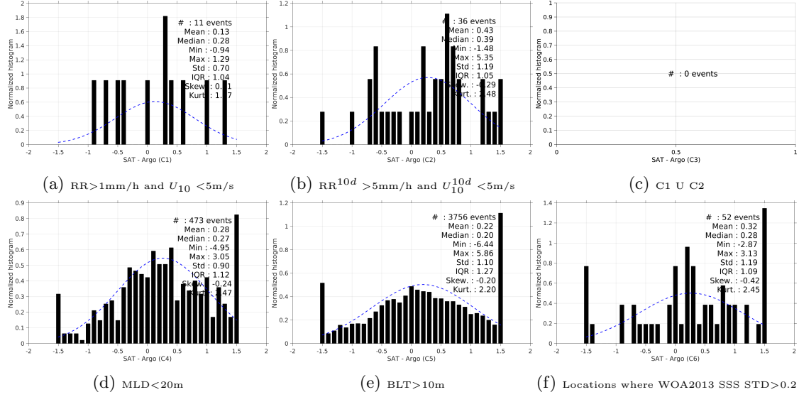
Figure 13: Normalized histogram of \Delta SSS (AQUARIUS-L2-JPL-V4 - Argo) for 6 different sub-datasets corresponding to: RR > 1\text{mm/h} and U_{10} < 5\text{m/s} (a), RR^{10d} > 5\text{mm/h} and U_{10}^{10d} < 5\text{m/s} (b), C1 U C2 (c), MLD < 20\text{m} (d), BLT > 10\text{m} (e), Locations where WOA2013 SSS STD > 0.2 (f).
