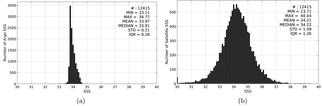
Figure 2: Histograms of SSS from Argo (a) and AQUARIUS-L2-JPL-V4 (b) considering all match-up pairs per bins of 0.1 over the Southern Ocean Pi-MEP region and for the full satellite product period.
