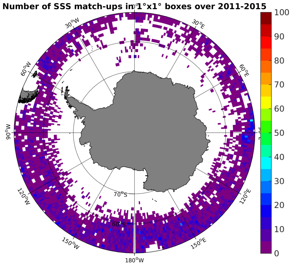
Figure 4: Number of SSS match-ups between Argo SSS and the AQUARIUS-L2-JPL-V4 SSS product for the Southern Ocean Pi-MEP region over 1^\circ \times 1^\circ boxes and for the full satellite product period.
