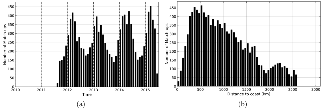
Figure 1: Number of match-ups between Argo and AQUARIUS-L2-JPL-V4 SSS as a function of time (a) and as function of the distance to coast (b) over the Southern Ocean Pi-MEP region and for the full satellite product period.
