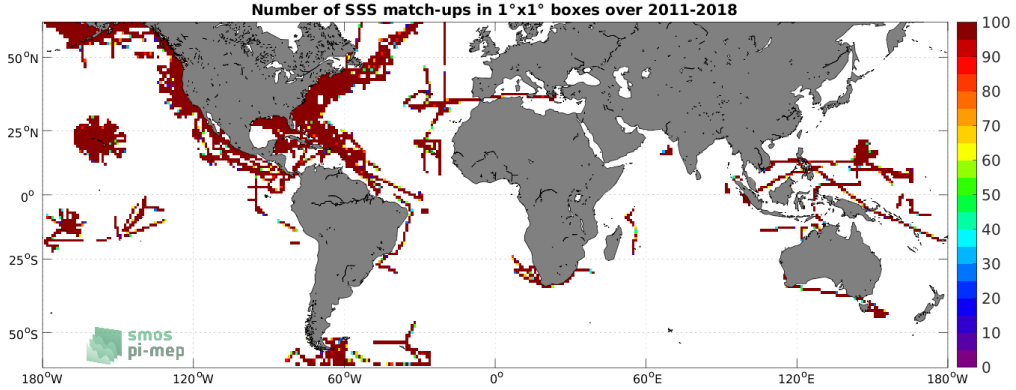
Figure 4: Number of SSS match-ups between TSG (SAMOS) SSS and the SMOS and SMAP SSS L4 OI v1 - 7 Days (LOPS) SSS product for the SMOS coastal zone (<800km) 60N-60S Pi-MEP region over 1^{\circ} \times 1^{\circ} boxes and for the full satellite product period.
