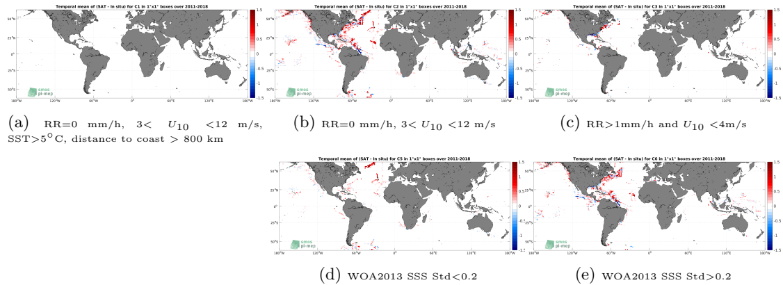
Figure 12: Temporal mean gridded over spatial boxes of size 1^\circ \times 1^\circ of \Delta SSS (SMOS and SMAP SSS L4 OI v1 - 7 Days (LOPS) - TSG (SAMOS)) for 5 different subdatasets corresponding to:RR=0 mm/h, 3 < U_{10} < 12 m/s, SST >5^\circ C, distance to coast > 800 km (a), RR=0 mm/h, 3 < U_{10} < 12 m/s (b), RR >1 mm/h and U_{10} < 4 m/s (c), WOA2013 SSS Std <0.2 (d), WOA2013 SSS Std >0.2 (e).
