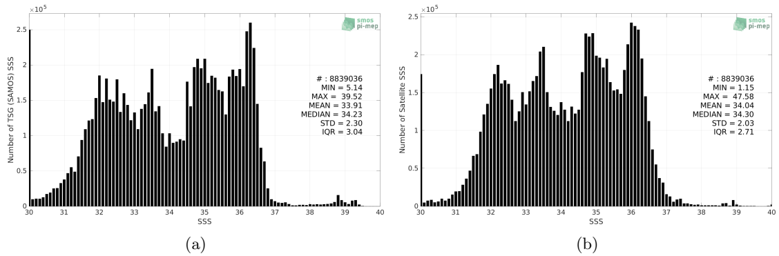
Figure 2: Histograms of SSS from TSG (SAMOS) (a) and SMOS and SMAP SSS L4 OI v1 - 7 Days (LOPS) (b) considering all match-up pairs per bins of 0.1 over the SMOS coastal zone (<800km) 60N-60S Pi-MEP region and for the full satellite product period.
