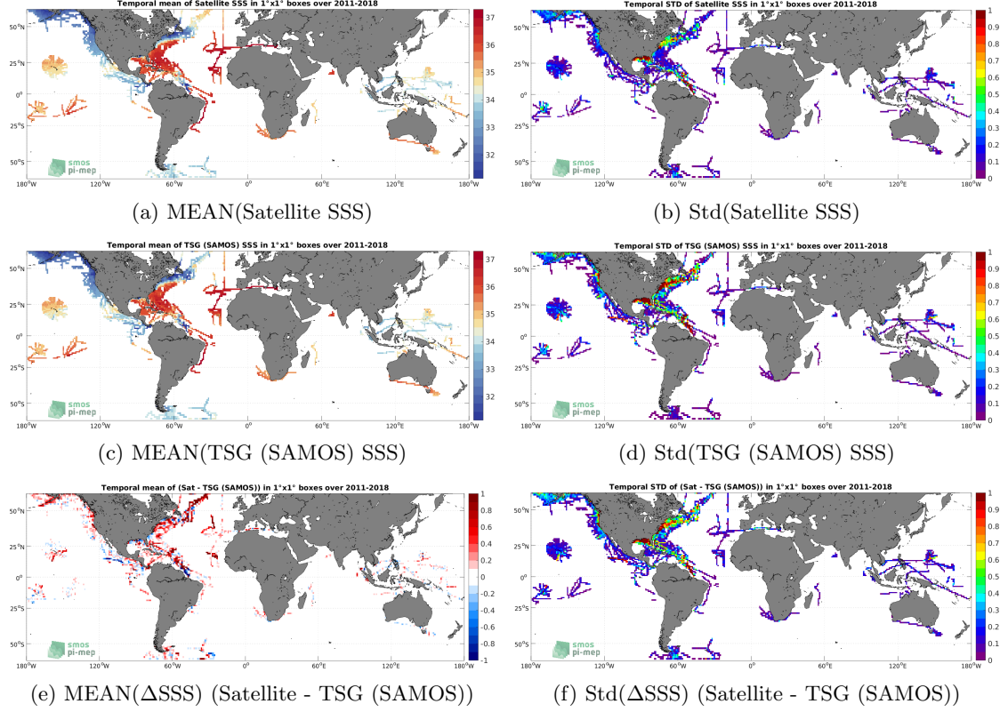
Figure 6: Temporal mean (left) and Std (right) of SSS from SMOS and SMAP SSS L4 OI v1 - 7 Days (LOPS) (top), TSG (SAMOS) (middle), and of \Delta SSS (Satellite - TSG (SAMOS)). Only match-up pairs are used to generate these maps.
