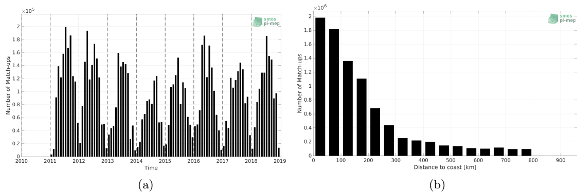
Figure 1: Number of match-ups between TSG (SAMOS) and SMOS and SMAP SSS L4 OI v1 - 7 Days (LOPS) SSS as a function of time (a) and as function of the distance to coast (b) over the SMOS coastal zone (<800km) 60N-60S Pi-MEP region and for the full satellite product period.
