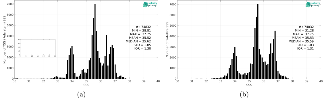
Figure 2: Histograms of SSS from TSG (Polarstern) (a) and SMOS and SMAP SSS L4 OI v1 - 7 Days (LOPS) (b) considering all match-up pairs per bins of 0.1 over the SMOS coastal zone (<800km) 60N-60S Pi-MEP region and for the full satellite product period.
