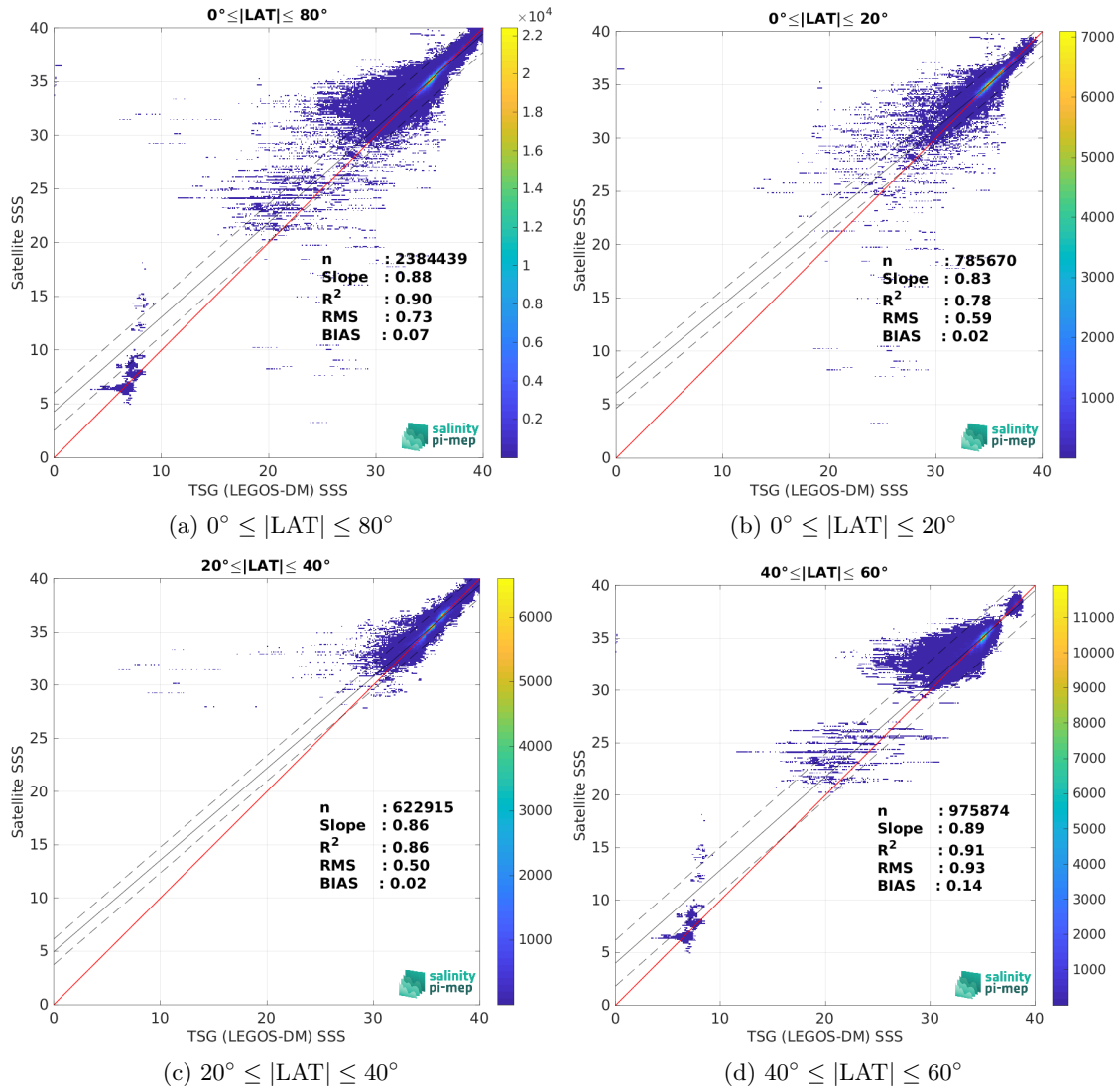
Figure 9: Contour maps of the concentration of SMOS and SMAP SSS L4 OI v1 - 7 Days (LOPS) SSS (y-axis) versus TSG (LEGOS-DM) SSS (x-axis) at match-up pairs for different latitude bands. For each plot, the red line shows x=y . The black thin and dashed lines indicate a linear fit through the data cloud and the \pm 95\% confidence levels, respectively. The number match-up pairs n , the slope and R^2 coefficient of the linear fit, the root mean square (RMS) and the mean bias between satellite and in situ data are indicated for each latitude band in each plots.
