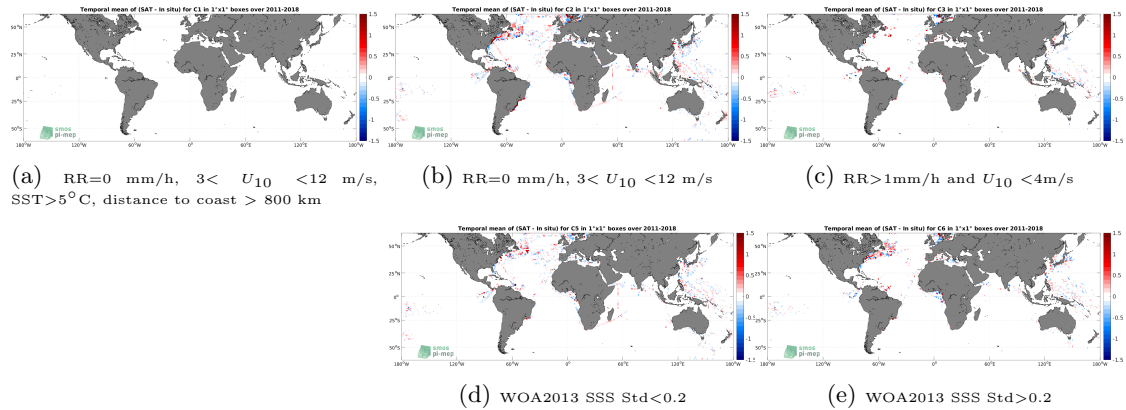
Figure 12: Temporal mean gridded over spatial boxes of size 1^\circ \times 1^\circ of \Delta\text{SSS} (SMOS and SMAP SSS L4 OI v1 - 7 Days (LOPS) - TSG (LEGOS-DM)) for 5 different subdatasets corresponding to:RR=0 mm/h, 3 < U_{10} < 12 m/s, SST >5^\circ\text{C} , distance to coast > 800 km (a), RR=0 mm/h, 3 < U_{10} < 12 m/s (b), RR >1 mm/h and U_{10} < 4 m/s (c), WOA2013 SSS Std <0.2 (d), WOA2013 SSS Std >0.2 (e).
