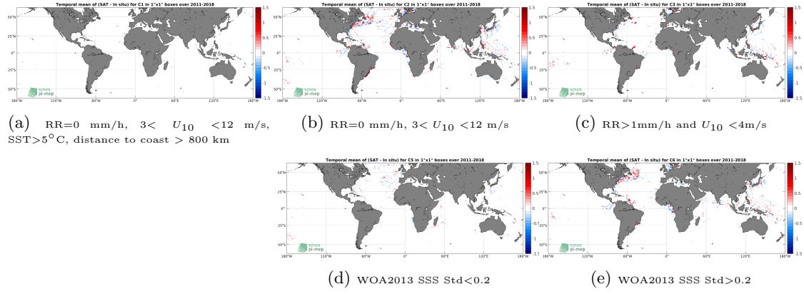
Figure 12: Temporal mean gridded over spatial boxes of size 1^\circ \times 1^\circ of \Delta SSS (SMOS and SMAP SSS L4 OI v1 - 7 Days (LOPS) - TSG (LEGOS-DM)) for 5 different subdatasets corresponding to:RR=0 mm/h, 3 < U_{10} < 12 m/s, SST >5^\circ C, distance to coast > 800 km (a), RR=0 mm/h, 3 < U_{10} < 12 m/s (b), RR >1 mm/h and U_{10} < 4 m/s (c), WOA2013 SSS Std <0.2 (d), WOA2013 SSS Std >0.2 (e).
