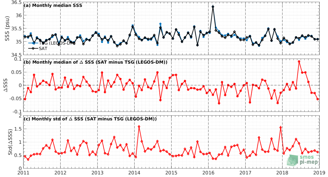
Figure 7: Time series of the monthly median SSS (top), median of \Delta\text{SSS} (Satellite - TSG (LEGOS-DM)) and Std of \Delta\text{SSS} (Satellite - TSG (LEGOS-DM)) over the SMOS coastal zone (<800km) 60N-60S Pi-MEP region considering all match-ups collected by the Pi-MEP.
