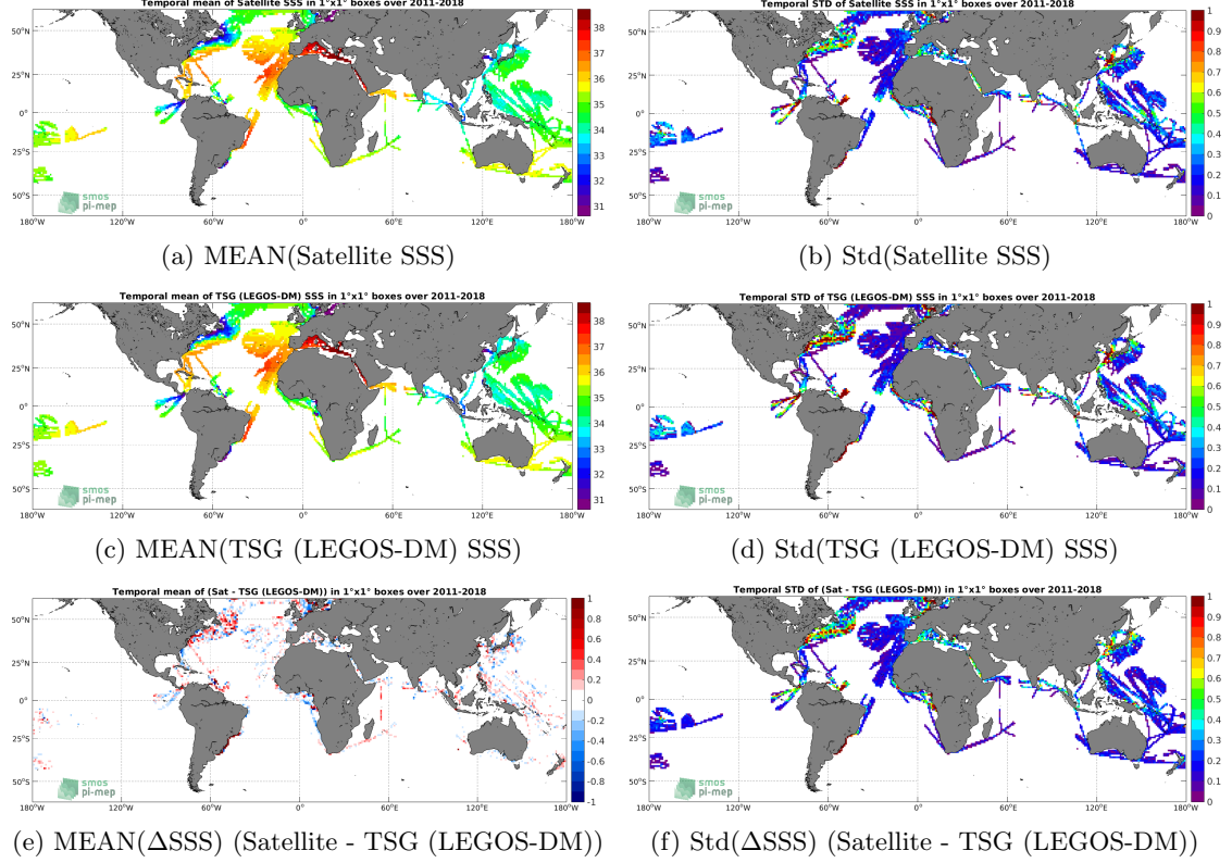
Figure 6: Temporal mean (left) and Std (right) of SSS from SMOS and SMAP SSS L4 OI v1 - 7 Days (LOPS) (top), TSG (LEGOS-DM) (middle), and of \Delta SSS (Satellite - TSG (LEGOS-DM)). Only match-up pairs are used to generate these maps.
