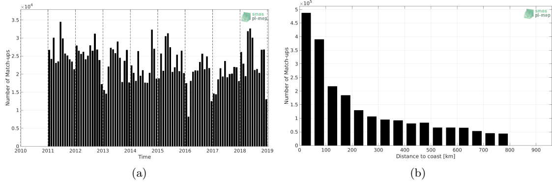
Figure 1: Number of match-ups between TSG (LEGOS-DM) and SMOS and SMAP SSS L4 OI v1 - 7 Days (LOPS) SSS as a function of time (a) and as function of the distance to coast (b) over the SMOS coastal zone (<800km) 60N-60S Pi-MEP region and for the full satellite product period.
