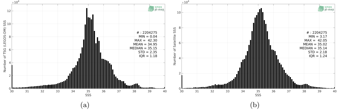
Figure 2: Histograms of SSS from TSG (LEGOS-DM) (a) and SMOS and SMAP SSS L4 OI v1 - 7 Days (LOPS) (b) considering all match-up pairs per bins of 0.1 over the SMOS coastal zone (<800km) 60N-60S Pi-MEP region and for the full satellite product period.
