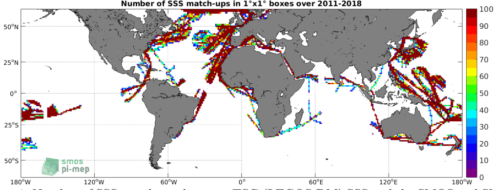
Figure 4: Number of SSS match-ups between TSG (LEGOS-DM) SSS and the SMOS and SMAP SSS L4 OI v1 - 7 Days (LOPS) SSS product for the SMOS coastal zone (<800km) 60N-60S Pi-MEP region over 1^\circ \times 1^\circ boxes and for the full satellite product period.
