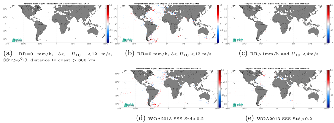
Figure 12: Temporal mean gridded over spatial boxes of size 1^\circ \times 1^\circ of \Delta\text{SSS} (SMOS and SMAP SSS L4 OI v1 - 7 Days (LOPS) - TSG (GOSUD-Sailing-ship)) for 5 different subdatasets corresponding to:RR=0 mm/h, 3 < U_{10} < 12 m/s, SST >5^\circ\text{C} , distance to coast > 800 km (a), RR=0 mm/h, 3 < U_{10} < 12 m/s (b), RR >1 mm/h and U_{10} < 4 m/s (c), WOA2013 SSS Std <0.2 (d), WOA2013 SSS Std >0.2 (e).
