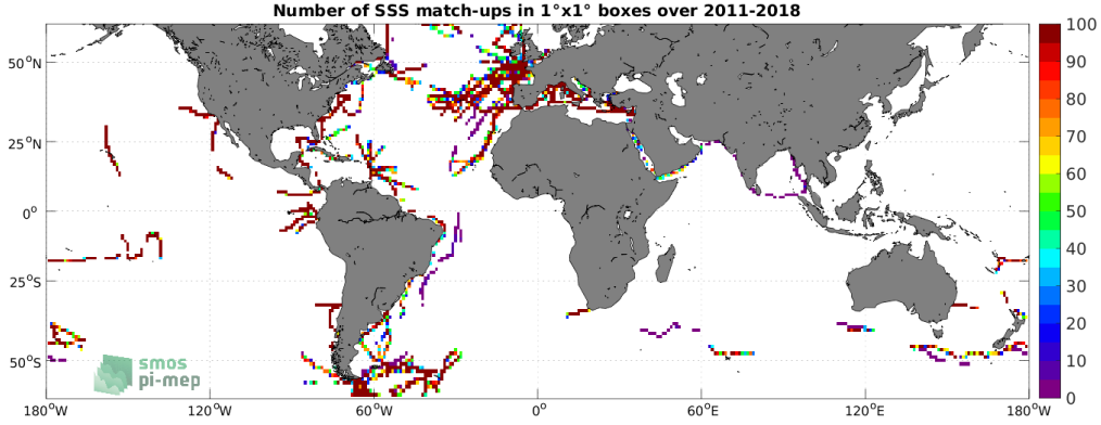
Figure 4: Number of SSS match-ups between TSG (GOSUD-Sailing-ship) SSS and the SMOS and SMAP SSS L4 OI v1 - 7 Days (LOPS) SSS product for the SMOS coastal zone (<800km) 60N-60S Pi-MEP region over 1^\circ \times 1^\circ boxes and for the full satellite product period.
