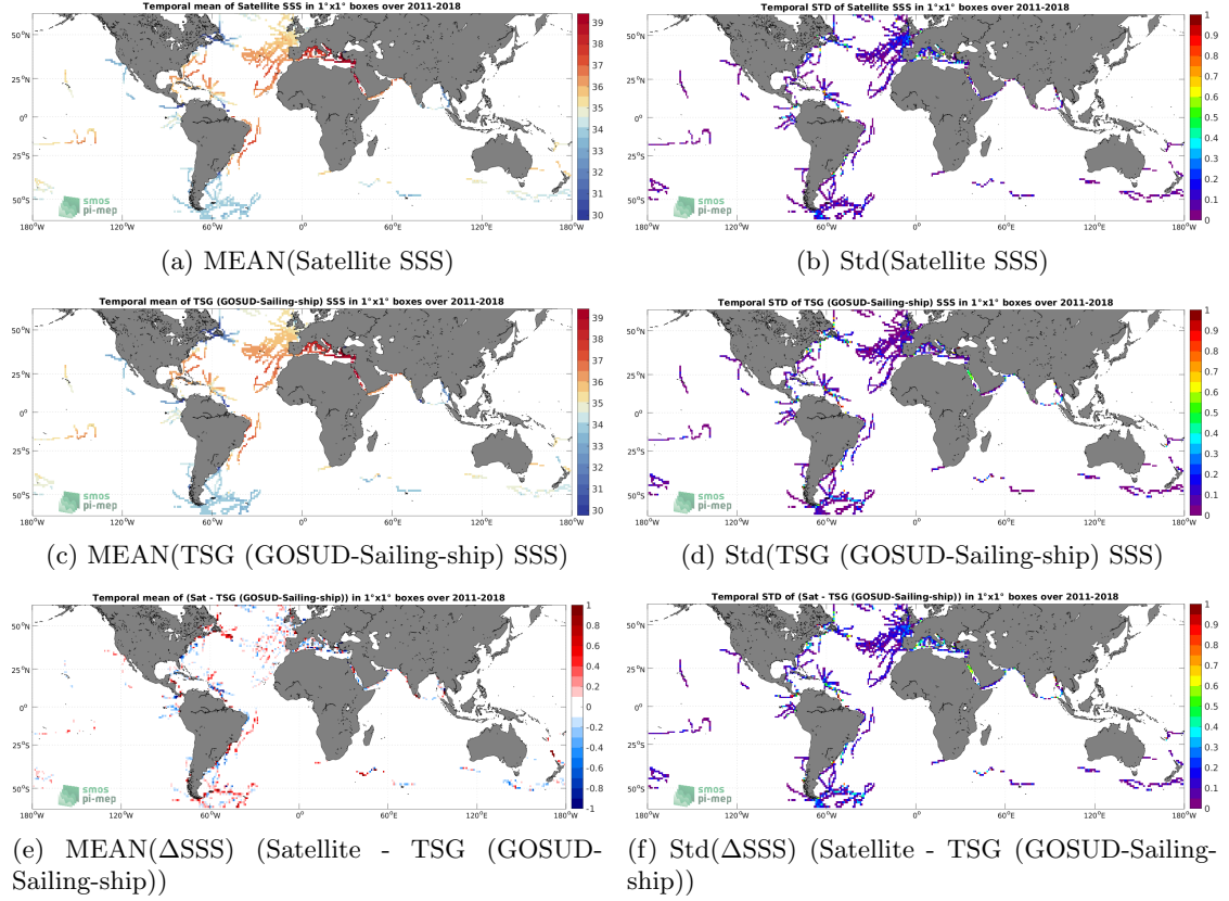
Figure 6: Temporal mean (left) and Std (right) of SSS from SMOS and SMAP SSS L4 OI v1 - 7 Days (LOPS) (top), TSG (GOSUD-Sailing-ship) (middle), and of \Delta SSS (Satellite - TSG (GOSUD-Sailing-ship)). Only match-up pairs are used to generate these maps.
