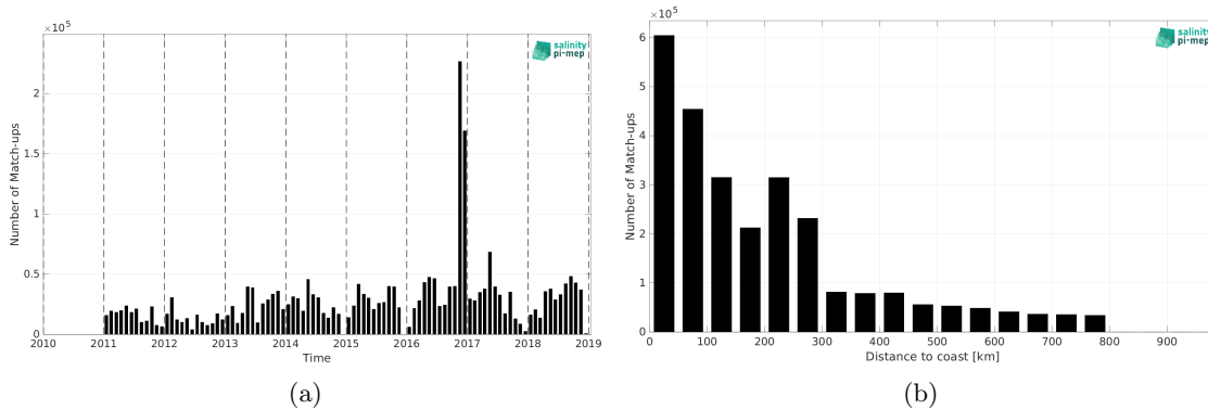
Figure 1: Number of match-ups between TSG (GOSUD-Research-vessel) and SMOS and SMAP SSS L4 OI v1 - 7 Days (LOPS) SSS as a function of time (a) and as function of the distance to coast (b) over the SMOS coastal zone (<800km) 60N-60S Pi-MEP region and for the full satellite product period.
