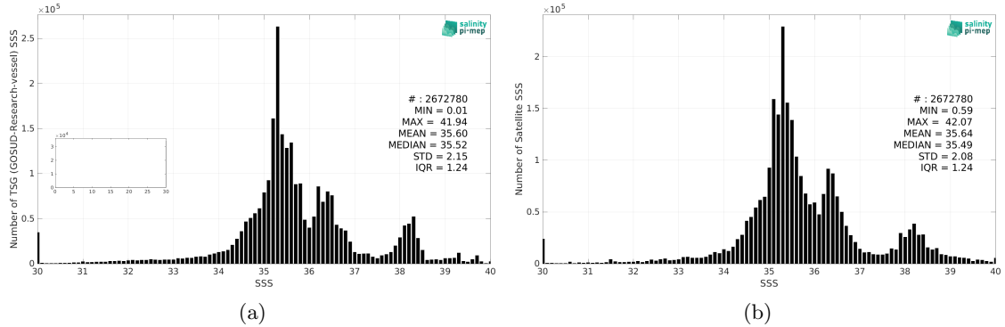
Figure 2: Histograms of SSS from TSG (GOSUD-Research-vessel) (a) and SMOS and SMAP SSS L4 OI v1 - 7 Days (LOPS) (b) considering all match-up pairs per bins of 0.1 over the SMOS coastal zone (<800km) 60N-60S Pi-MEP region and for the full satellite product period.
