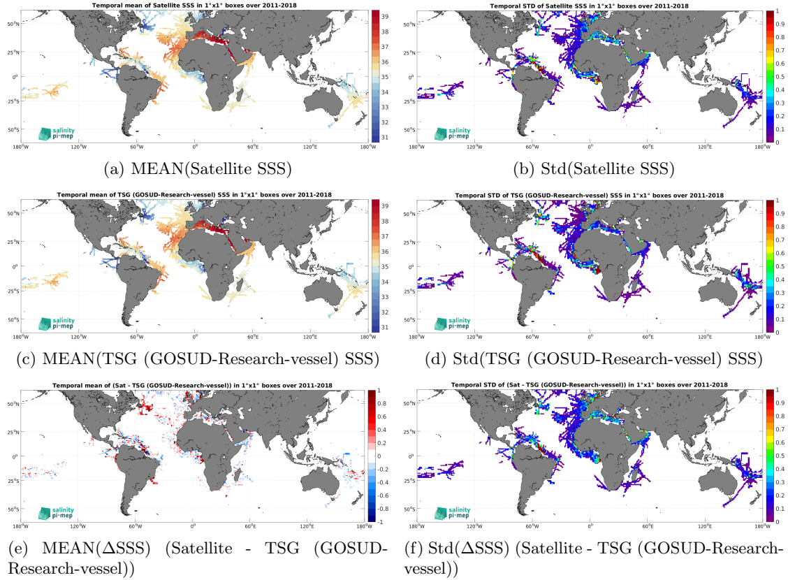
Figure 6: Temporal mean (left) and Std (right) of SSS from SMOS and SMAP SSS L4 OI v1 - 7 Days (LOPS) (top), TSG (GOSUD-Research-vessel) (middle), and of \Delta\text{SSS} (Satellite - TSG (GOSUD-Research-vessel)). Only match-up pairs are used to generate these maps.
