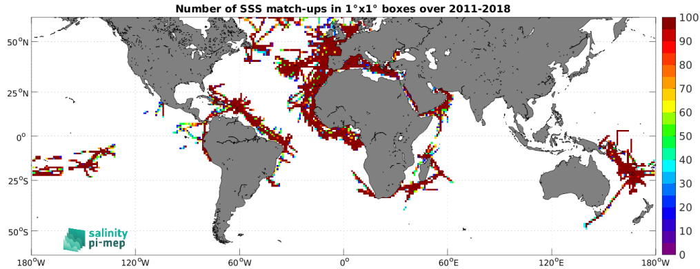
Figure 4: Number of SSS match-ups between TSG (GOSUD-Research-vessel) SSS and the SMOS and SMAP SSS L4 OI v1 - 7 Days (LOPS) SSS product for the SMOS coastal zone ( <800\text{km} ) 60N-60S Pi-MEP region over 1^\circ \times 1^\circ boxes and for the full satellite product period.
