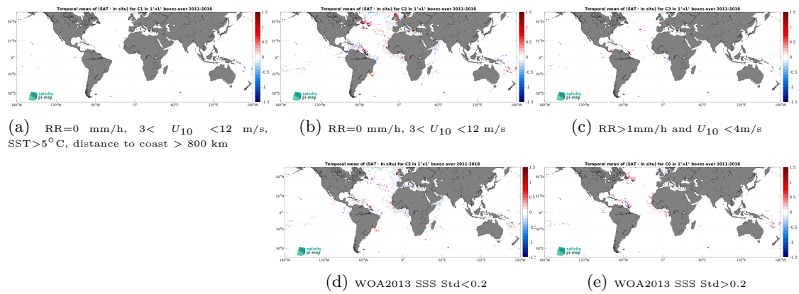
Figure 12: Temporal mean gridded over spatial boxes of size 1^\circ \times 1^\circ of \Delta SSS (SMOS and SMAP SSS L4 OI v1 - 7 Days (LOPS) - TSG (GOSUD-Research-vessel)) for 5 different subdatasets corresponding to:RR=0 mm/h, 3 < U_{10} < 12 m/s, SST >5^\circ\text{C} , distance to coast > 800 km (a), RR=0 mm/h, 3 < U_{10} < 12 m/s (b), RR >1 mm/h and U_{10} < 4 m/s (c), WOA2013 SSS Std <0.2 (d), WOA2013 SSS Std >0.2 (e).
