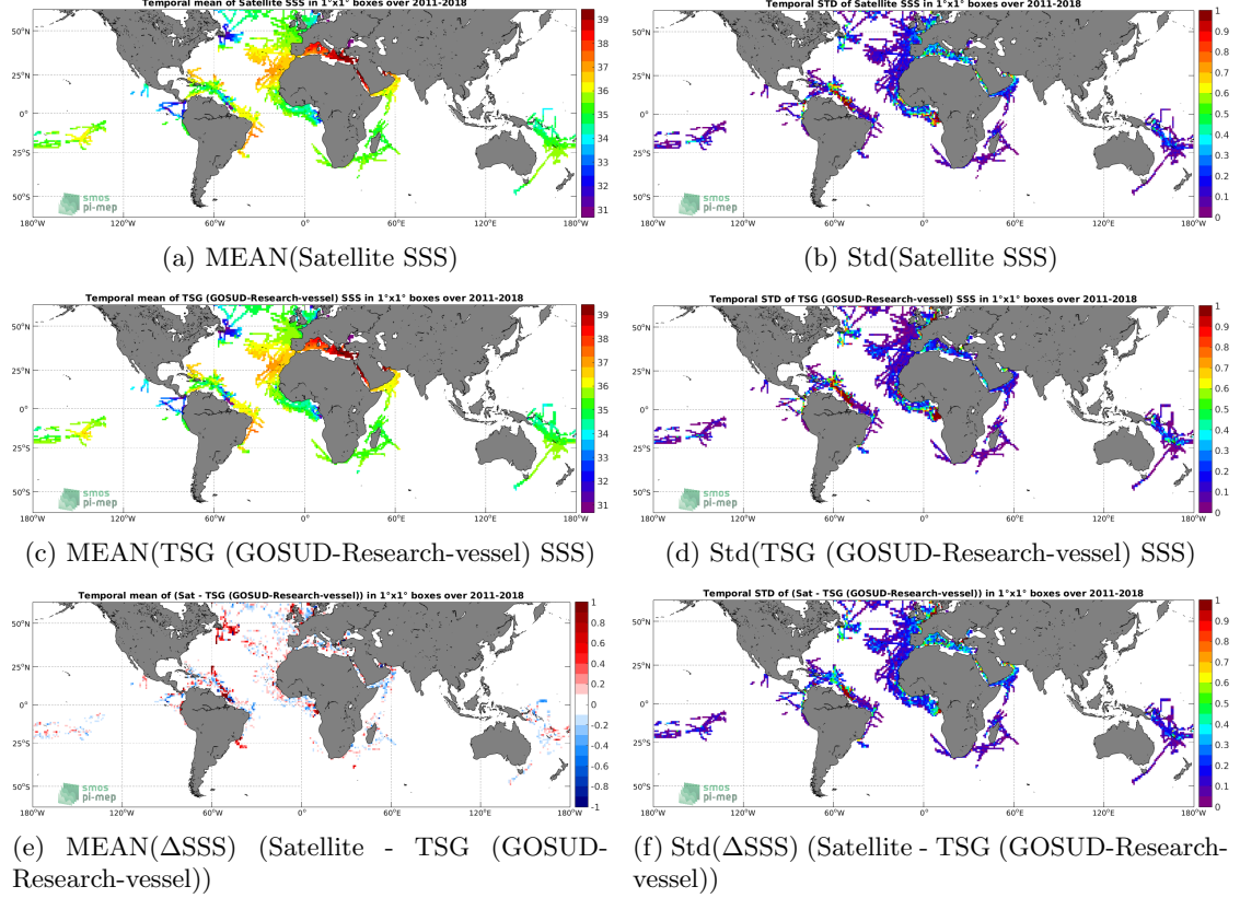
Figure 6: Temporal mean (left) and Std (right) of SSS from SMOS and SMAP SSS L4 OI v1 - 7 Days (LOPS) (top), TSG (GOSUD-Research-vessel) (middle), and of \Delta SSS (Satellite - TSG (GOSUD-Research-vessel)). Only match-up pairs are used to generate these maps.
