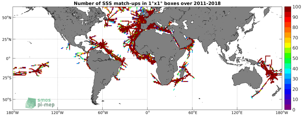
Figure 4: Number of SSS match-ups between TSG (GOSUD-Research-vessel) SSS and the SMOS and SMAP SSS L4 OI v1 - 7 Days (LOPS) SSS product for the SMOS coastal zone (<800km) 60N-60S Pi-MEP region over 1^\circ \times 1^\circ boxes and for the full satellite product period.
