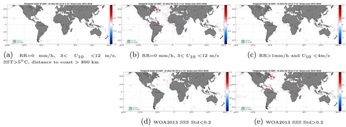
Figure 12: Temporal mean gridded over spatial boxes of size 1^\circ \times 1^\circ of \Delta\text{SSS} (SMOS and SMAP SSS L4 OI v1 - 7 Days (LOPS) - TSG (GOSUD-Research-vessel)) for 5 different subdatasets corresponding to:RR=0 mm/h, 3 < U_{10} < 12 m/s, SST>5°C, distance to coast > 800 km (a), RR=0 mm/h, 3 < U_{10} < 12 m/s (b), RR>1mm/h and U_{10} < 4 m/s (c), WOA2013 SSS Std<0.2 (d), WOA2013 SSS Std>0.2 (e).
