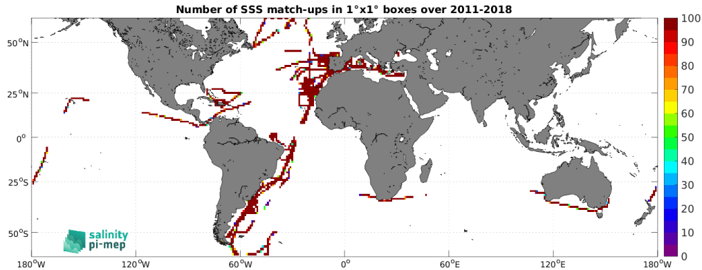
Figure 4: Number of SSS match-ups between TSG (CSIC-UTM) SSS and the SMOS and SMAP SSS L4 OI v1 - 7 Days (LOPS) SSS product for the SMOS coastal zone (<800km) 60N-60S Pi-MEP region over 1^\circ \times 1^\circ boxes and for the full satellite product period.
