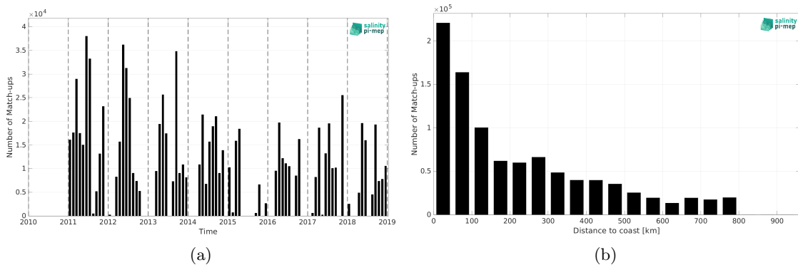
Figure 1: Number of match-ups between TSG (CSIC-UTM) and SMOS and SMAP SSS L4 OI v1 - 7 Days (LOPS) SSS as a function of time (a) and as function of the distance to coast (b) over the SMOS coastal zone (<800km) 60N-60S Pi-MEP region and for the full satellite product period.
