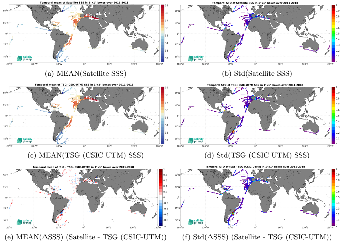
Figure 6: Temporal mean (left) and Std (right) of SSS from SMOS and SMAP SSS L4 OI v1 - 7 Days (LOPS) (top), TSG (CSIC-UTM) (middle), and of \Delta SSS (Satellite - TSG (CSIC-UTM)). Only match-up pairs are used to generate these maps.
