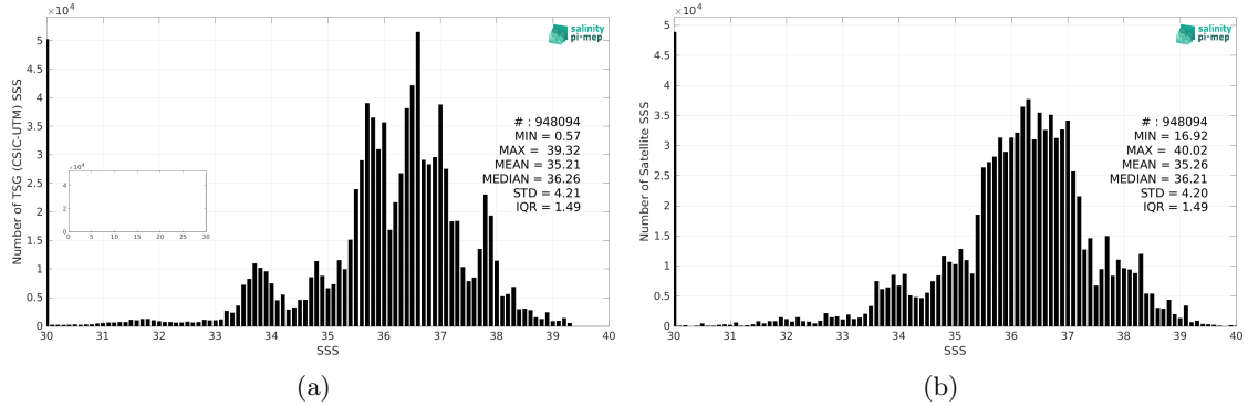
Figure 2: Histograms of SSS from TSG (CSIC-UTM) (a) and SMOS and SMAP SSS L4 OI v1 - 7 Days (LOPS) (b) considering all match-up pairs per bins of 0.1 over the SMOS coastal zone (<800km) 60N-60S Pi-MEP region and for the full satellite product period.
