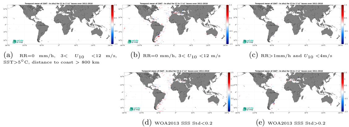
Figure 12: Temporal mean gridded over spatial boxes of size 1^\circ \times 1^\circ of \Delta SSS (SMOS and SMAP SSS L4 OI v1 - 7 Days (LOPS) - TSG (CSIC-UTM)) for 5 different subdatasets corresponding to:RR=0 mm/h, 3 < U_{10} < 12 m/s, SST >5^\circ C, distance to coast > 800 km (a), RR=0 mm/h, 3 < U_{10} < 12 m/s (b), RR >1 mm/h and U_{10} < 4 m/s (c), WOA2013 SSS Std <0.2 (d), WOA2013 SSS Std >0.2 (e).
