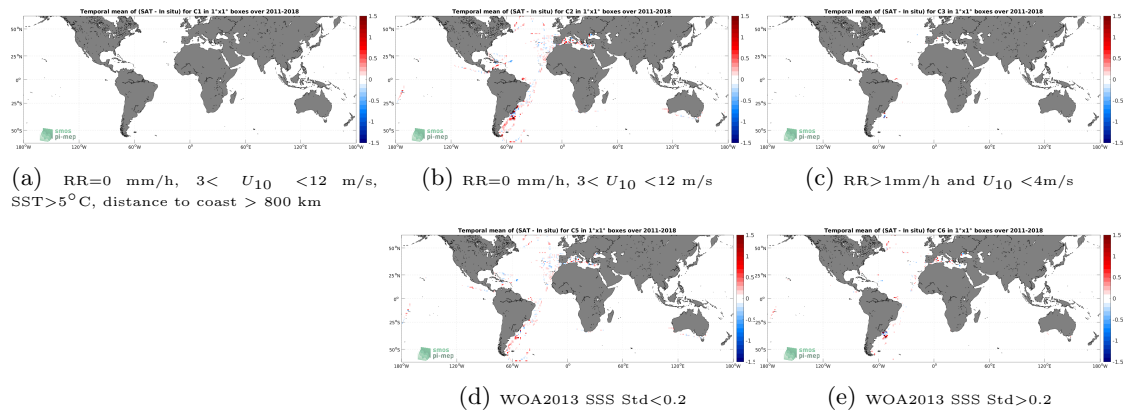
Figure 12: Temporal mean gridded over spatial boxes of size 1^\circ \times 1^\circ of \Delta\text{SSS} (SMOS and SMAP SSS L4 OI v1 - 7 Days (LOPS) - TSG (CSIC-UTM)) for 5 different subdatasets corresponding to:RR=0 mm/h, 3 < U_{10} < 12 m/s, SST >5^\circ\text{C} , distance to coast > 800 km (a), RR=0 mm/h, 3 < U_{10} < 12 m/s (b), RR >1 mm/h and U_{10} < 4 m/s (c), WOA2013 SSS Std <0.2 (d), WOA2013 SSS Std >0.2 (e).
