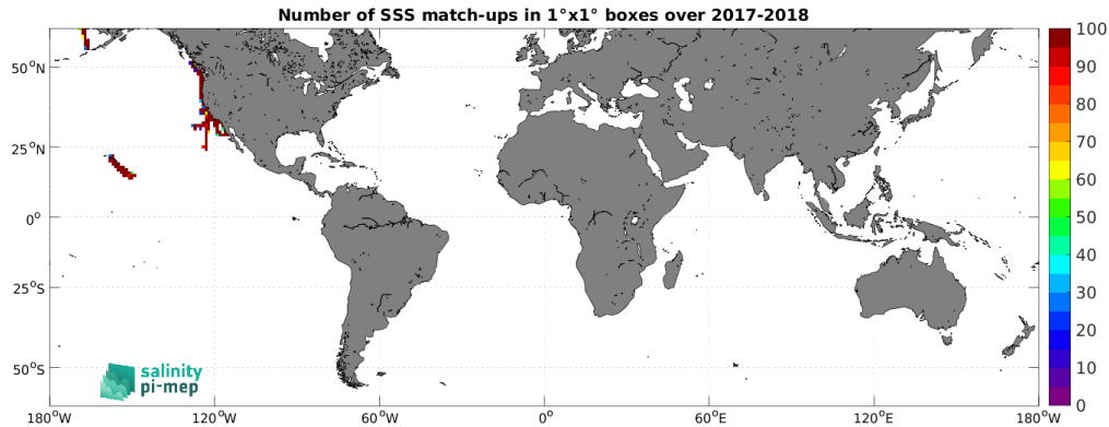
Figure 4: Number of SSS match-ups between Saildrone SSS and the SMOS and SMAP SSS L4 OI v1 - 7 Days (LOPS) SSS product for the SMOS coastal zone (<800km) 60N-60S Pi-MEP region over 1^\circ \times 1^\circ boxes and for the full satellite product period.
