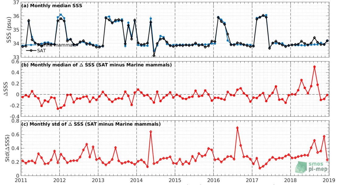
Figure 7: Time series of the monthly median SSS (top), median of \Delta SSS (Satellite - Marine mammals) and Std of \Delta SSS (Satellite - Marine mammals) over the SMOS coastal zone ( <800\text{km} ) 60N-60S Pi-MEP region considering all match-ups collected by the Pi-MEP.
