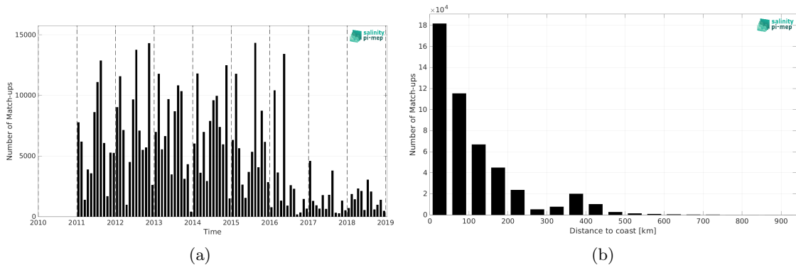
Figure 1: Number of match-ups between ICES and SMOS and SMAP SSS L4 OI v1 - 7 Days (LOPS) SSS as a function of time (a) and as function of the distance to coast (b) over the SMOS coastal zone ( < 800\text{km} ) 60N-60S Pi-MEP region and for the full satellite product period.
