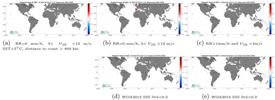
Figure 12: Temporal mean gridded over spatial boxes of size 1^\circ \times 1^\circ of \Delta SSS (SMOS and SMAP SSS L4 OI v1 - 7 Days (LOPS) - ICES) for 5 different subdatasets corresponding to:RR=0 mm/h, 3 < U_{10} < 12 m/s, SST >5^\circ\text{C} , distance to coast > 800 km (a), RR=0 mm/h, 3 < U_{10} < 12 m/s (b), RR >1 mm/h and U_{10} < 4 m/s (c), WOA2013 SSS Std <0.2 (d), WOA2013 SSS Std >0.2 (e).
