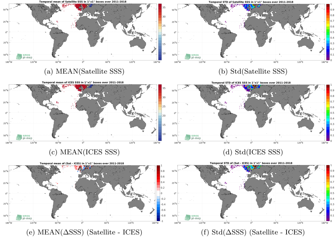
Figure 6: Temporal mean (left) and Std (right) of SSS from SMOS and SMAP SSS L4 OI v1 - 7 Days (LOPS) (top), ICES (middle), and of \Delta SSS (Satellite - ICES). Only match-up pairs are used to generate these maps.
