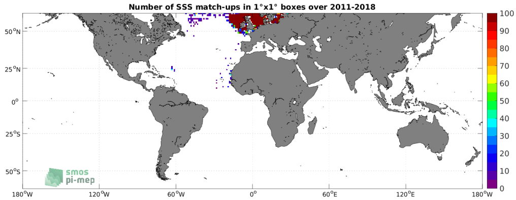
Figure 4: Number of SSS match-ups between ICES SSS and the SMOS and SMAP SSS L4 OI v1 - 7 Days (LOPS) SSS product for the SMOS coastal zone (<800km) 60N-60S Pi-MEP region over 1^\circ \times 1^\circ boxes and for the full satellite product period.
