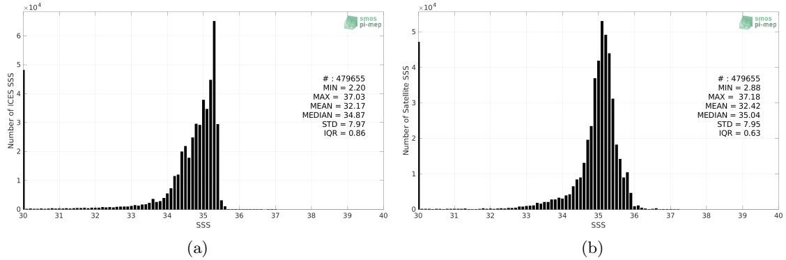
Figure 2: Histograms of SSS from ICES (a) and SMOS and SMAP SSS L4 OI v1 - 7 Days (LOPS) (b) considering all match-up pairs per bins of 0.1 over the SMOS coastal zone (<800km) 60N-60S Pi-MEP region and for the full satellite product period.
