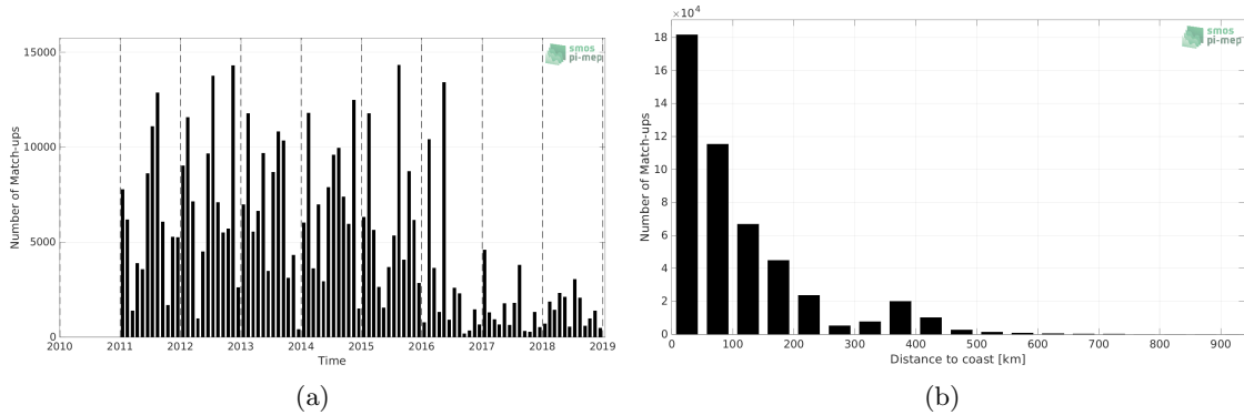
Figure 1: Number of match-ups between ICES and SMOS and SMAP SSS L4 OI v1 - 7 Days (LOPS) SSS as a function of time (a) and as function of the distance to coast (b) over the SMOS coastal zone (<800km) 60N-60S Pi-MEP region and for the full satellite product period.
