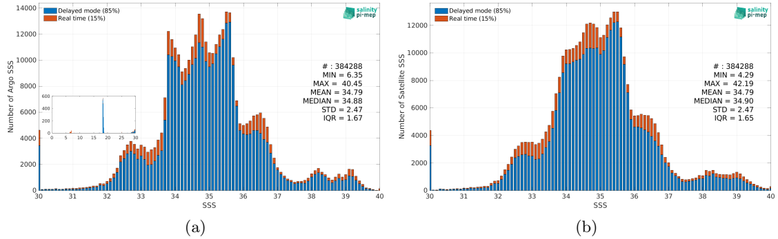
Figure 2: Histograms of SSS from Argo (a) and SMOS and SMAP SSS L4 OI v1 - 7 Days (LOPS) (b) considering all match-up pairs per bins of 0.1 over the SMOS coastal zone (<800km) 60N-60S Pi-MEP region and for the full satellite product period.
