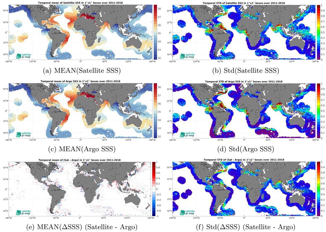
Figure 6: Temporal mean (left) and Std (right) of SSS from SMOS and SMAP SSS L4 OI v1 - 7 Days (LOPS) (top), Argo (middle), and of \Delta SSS (Satellite - Argo). Only match-up pairs are used to generate these maps.
