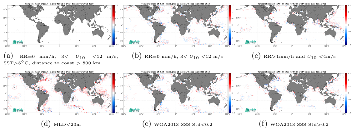
Figure 12: Temporal mean gridded over spatial boxes of size 1^\circ \times 1^\circ of \Delta SSS (SMOS and SMAP SSS L4 OI v1 - 7 Days (LOPS) - Argo) for 6 different subdatasets corresponding to:RR=0 mm/h, 3 < U_{10} < 12 m/s, SST >5^\circ C, distance to coast > 800 km (a), RR=0 mm/h, 3 < U_{10} < 12 m/s (b), RR >1 mm/h and U_{10} < 4 m/s (c),MLD <20 m (d),WOA2013 SSS Std <0.2 (e),WOA2013 SSS Std >0.2 (f).
