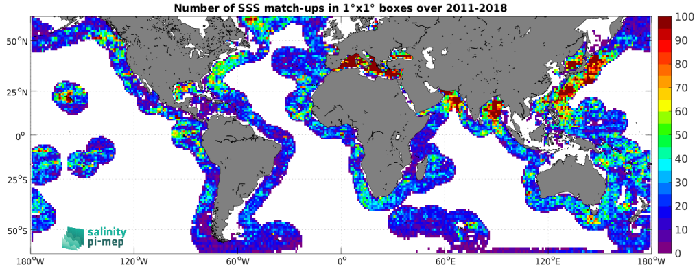
Figure 4: Number of SSS match-ups between Argo SSS and the SMOS and SMAP SSS L4 OI v1 - 7 Days (LOPS) SSS product for the SMOS coastal zone (<800km) 60N-60S Pi-MEP region over 1^{\circ} \times 1^{\circ} boxes and for the full satellite product period.
