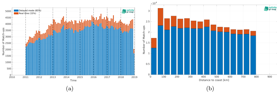
Figure 1: Number of match-ups between Argo and SMOS and SMAP SSS L4 OI v1 - 7 Days (LOPS) SSS as a function of time (a) and as function of the distance to coast (b) over the SMOS coastal zone (<800km) 60N-60S Pi-MEP region and for the full satellite product period.
