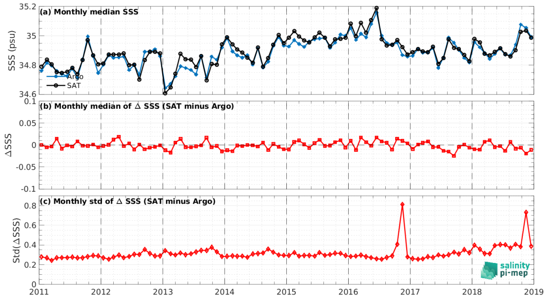
Figure 7: Time series of the monthly median SSS (top), median of \Delta SSS (Satellite - Argo) and Std of \Delta SSS (Satellite - Argo) over the SMOS coastal zone ( <800\text{km} ) 60N-60S Pi-MEP region considering all match-ups collected by the Pi-MEP.
