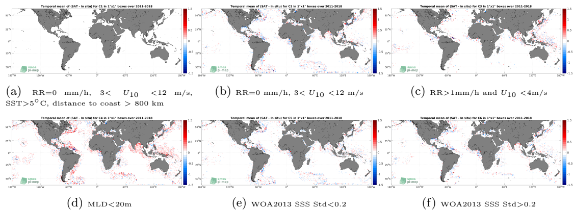
Figure 12: Temporal mean gridded over spatial boxes of size 1^\circ \times 1^\circ of \Delta SSS (SMOS and SMAP SSS L4 OI v1 - 7 Days (LOPS) - Argo) for 6 different subdatasets corresponding to: RR=0 mm/h, 3 < U_{10} < 12 m/s, SST > 5^\circ\text{C} , distance to coast > 800 km (a), RR=0 mm/h, 3 < U_{10} < 12 m/s (b), RR > 1 mm/h and U_{10} < 4 m/s (c),MLD < 20 m (d),WOA2013 SSS Std < 0.2 (e),WOA2013 SSS Std > 0.2 (f).
