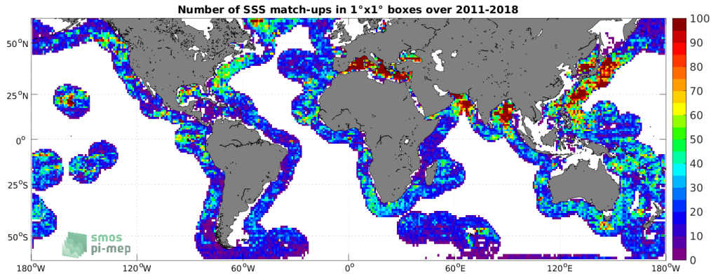
Figure 4: Number of SSS match-ups between Argo SSS and the SMOS and SMAP SSS L4 OI v1 - 7 Days (LOPS) SSS product for the SMOS coastal zone (<800km) 60N-60S Pi-MEP region over 1^\circ \times 1^\circ boxes and for the full satellite product period.
