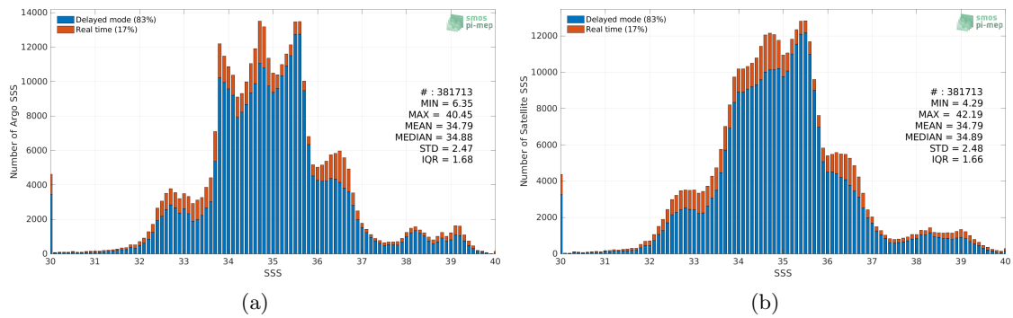
Figure 2: Histograms of SSS from Argo (a) and SMOS and SMAP SSS L4 OI v1 - 7 Days (LOPS) (b) considering all match-up pairs per bins of 0.1 over the SMOS coastal zone (<800km) 60N-60S Pi-MEP region and for the full satellite product period.
