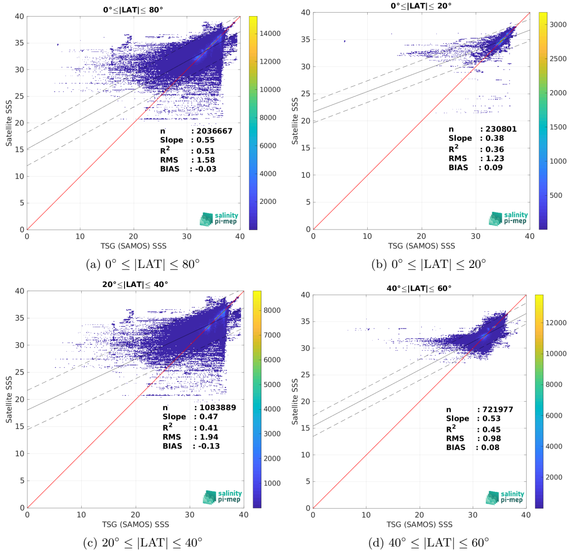
Figure 9: Contour maps of the concentration of SMOS SSS L4 v1 - Weekly (CMEMS-CNR) SSS (y-axis) versus TSG (SAMOS) SSS (x-axis) at match-up pairs for different latitude bands. For each plot, the red line shows x=y . The black thin and dashed lines indicate a linear fit through the data cloud and the \pm 95\% confidence levels, respectively. The number match-up pairs n , the slope and R^2 coefficient of the linear fit, the root mean square (RMS) and the mean bias between satellite and in situ data are indicated for each latitude band in each plot.
