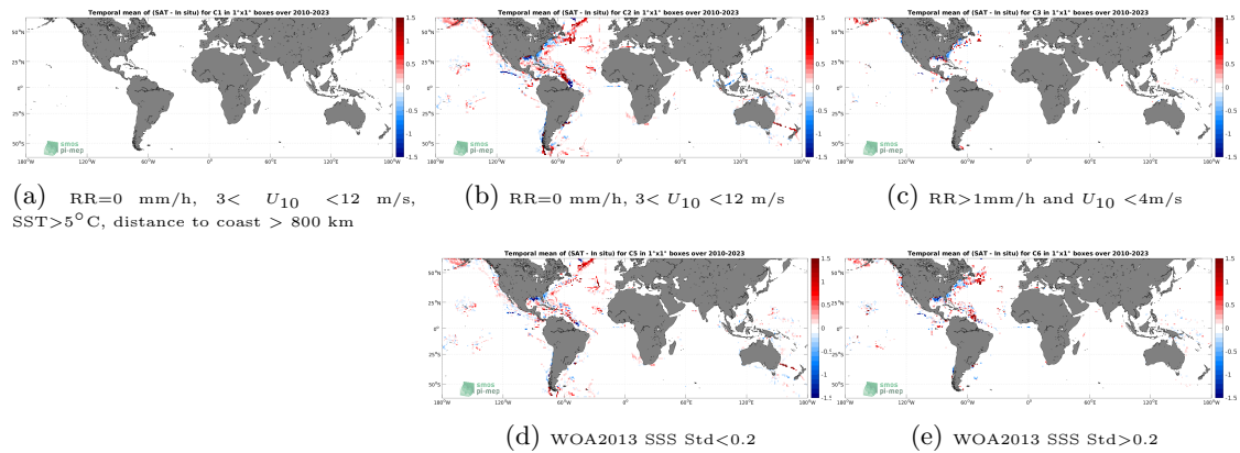
Figure 12: Temporal mean gridded over spatial boxes of size 1^\circ \times 1^\circ of \Delta SSS (SMOS SSS L4 v1 - Weekly (CMEMS-CNR) - TSG (SAMOS)) for 5 different subdatasets corresponding to:RR=0 mm/h, 3 < U_{10} < 12 m/s, SST >5^\circ C, distance to coast > 800 km (a), RR=0 mm/h, 3 < U_{10} < 12 m/s (b), RR >1 mm/h and U_{10} < 4 m/s (c), WOA2013 SSS Std <0.2 (d), WOA2013 SSS Std >0.2 (e).
