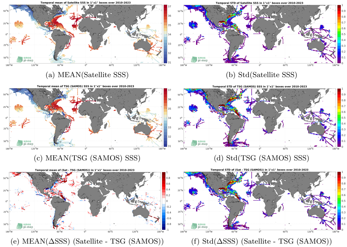
Figure 6: Temporal mean (left) and Std (right) of SSS from SMOS SSS L4 v1 - Weekly (CMEMS-CNR) (top), TSG (SAMOS) (middle), and of \Delta SSS (Satellite - TSG (SAMOS)). Only match-up pairs are used to generate these maps.
