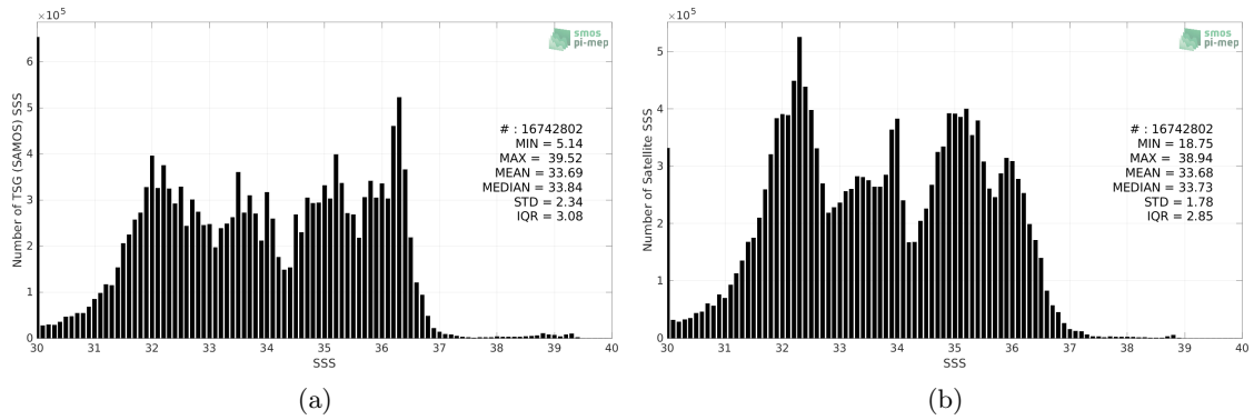
Figure 2: Histograms of SSS from TSG (SAMOS) (a) and SMOS SSS L4 v1 - Weekly (CMEMS-CNR) (b) considering all match-up pairs per bins of 0.1 over the SMOS coastal zone (<800km) 60N-60S Pi-MEP region and for the full satellite product period.
