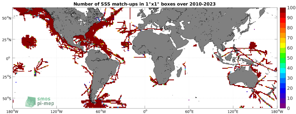
Figure 4: Number of SSS match-ups between TSG (SAMOS) SSS and the SMOS SSS L4 v1 - Weekly (CMEMS-CNR) SSS product for the SMOS coastal zone (<800km) 60N-60S Pi-MEP region over 1^{\circ} \times 1^{\circ} boxes and for the full satellite product period.
