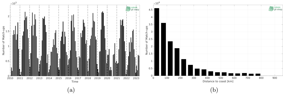
Figure 1: Number of match-ups between TSG (SAMOS) and SMOS SSS L4 v1 - Weekly (CMEMS-CNR) SSS as a function of time (a) and as function of the distance to coast (b) over the SMOS coastal zone (<800km) 60N-60S Pi-MEP region and for the full satellite product period.
