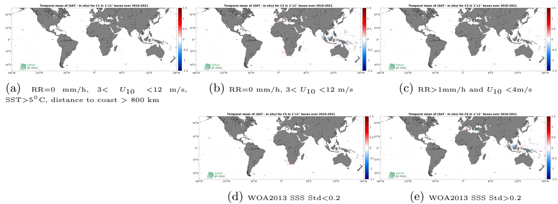
Figure 12: Temporal mean gridded over spatial boxes of size 1^\circ \times 1^\circ of \Delta\text{SSS} (SMOS SSS L4 v1 - Weekly (CMEMS-CNR) - TSG (SAMOS)) for 5 different subdatasets corresponding to:RR=0 mm/h, 3 < U_{10} < 12 m/s, SST >5^\circ\text{C} , distance to coast > 800 km (a), RR=0 mm/h, 3 < U_{10} < 12 m/s (b), RR >1 mm/h and U_{10} < 4 m/s (c), WOA2013 SSS Std <0.2 (d), WOA2013 SSS Std >0.2 (e).
