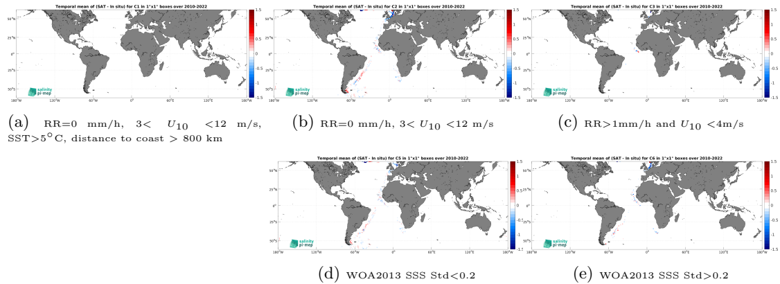
Figure 12: Temporal mean gridded over spatial boxes of size 1^\circ \times 1^\circ of \Delta\text{SSS} (SMOS SSS L4 v1 - Weekly (CMEMS-CNR) - TSG (Polarstern)) for 5 different subdatasets corresponding to:RR=0 mm/h, 3 < U_{10} < 12 m/s, SST >5^\circ\text{C} , distance to coast > 800 km (a), RR=0 mm/h, 3 < U_{10} < 12 m/s (b), RR >1 mm/h and U_{10} < 4 m/s (c), WOA2013 SSS Std <0.2 (d), WOA2013 SSS Std >0.2 (e).
