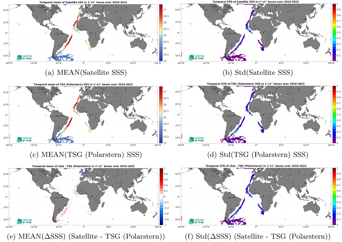
Figure 6: Temporal mean (left) and Std (right) of SSS from SMOS SSS L4 v1 - Weekly (CMEMS-CNR) (top), TSG (Polarstern) (middle), and of \Delta SSS (Satellite - TSG (Polarstern)). Only match-up pairs are used to generate these maps.
