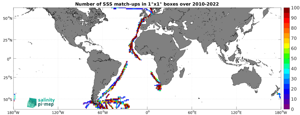
Figure 4: Number of SSS match-ups between TSG (Polarstern) SSS and the SMOS SSS L4 v1 - Weekly (CMEMS-CNR) SSS product for the SMOS coastal zone (<800km) 60N-60S Pi-MEP region over 1^{\circ} \times 1^{\circ} boxes and for the full satellite product period.
