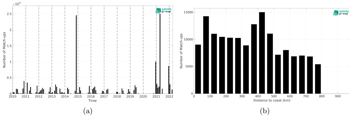
Figure 1: Number of match-ups between TSG (Polarstern) and SMOS SSS L4 v1 - Weekly (CMEMS-CNR) SSS as a function of time (a) and as function of the distance to coast (b) over the SMOS coastal zone (<800km) 60N-60S Pi-MEP region and for the full satellite product period.
