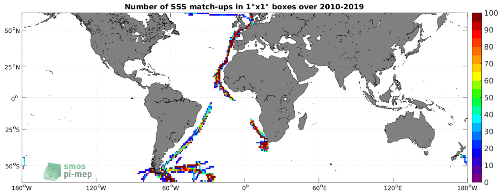
Figure 4: Number of SSS match-ups between TSG (Polarstern) SSS and the SMOS SSS L4 v1 - Weekly (CMEMS-CNR) SSS product for the SMOS coastal zone (<800km) 60N-60S Pi-MEP region over 1^\circ \times 1^\circ boxes and for the full satellite product period.
