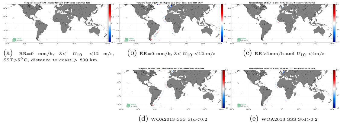
Figure 12: Temporal mean gridded over spatial boxes of size 1^\circ \times 1^\circ of \Delta SSS (SMOS SSS L4 v1 - Weekly (CMEMS-CNR) - TSG (Polarstern)) for 5 different subdatasets corresponding to:RR=0 mm/h, 3 < U_{10} < 12 m/s, SST >5^\circ\text{C} , distance to coast > 800 km (a), RR=0 mm/h, 3 < U_{10} < 12 m/s (b), RR >1 mm/h and U_{10} < 4 m/s (c), WOA2013 SSS Std <0.2 (d), WOA2013 SSS Std >0.2 (e).
