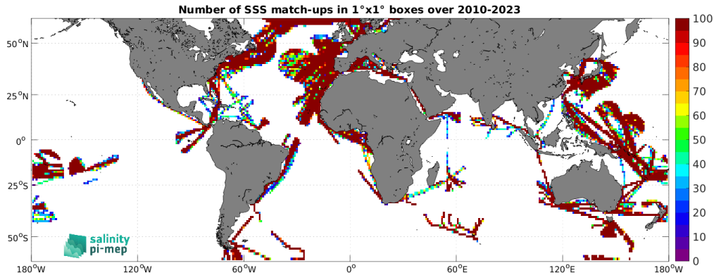
Figure 4: Number of SSS match-ups between TSG (LEGOS-DM) SSS and the SMOS SSS L4 v1 - Weekly (CMEMS-CNR) SSS product for the SMOS coastal zone (<800km) 60N-60S Pi-MEP region over 1^{\circ} \times 1^{\circ} boxes and for the full satellite product period.
