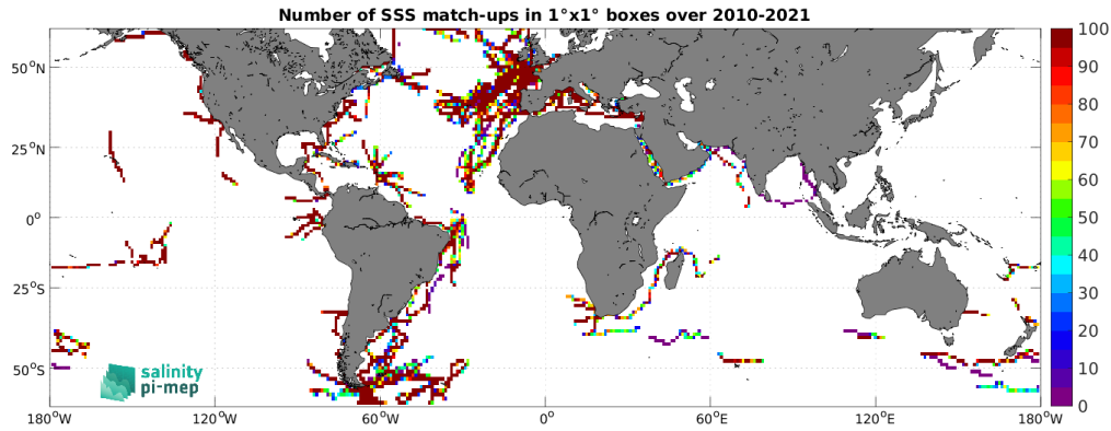
Figure 4: Number of SSS match-ups between TSG (GOSUD-Sailing-ship) SSS and the SMOS SSS L4 v1 - Weekly (CMEMS-CNR) SSS product for the SMOS coastal zone (<800km) 60N-60S Pi-MEP region over 1^{\circ} \times 1^{\circ} boxes and for the full satellite product period.
