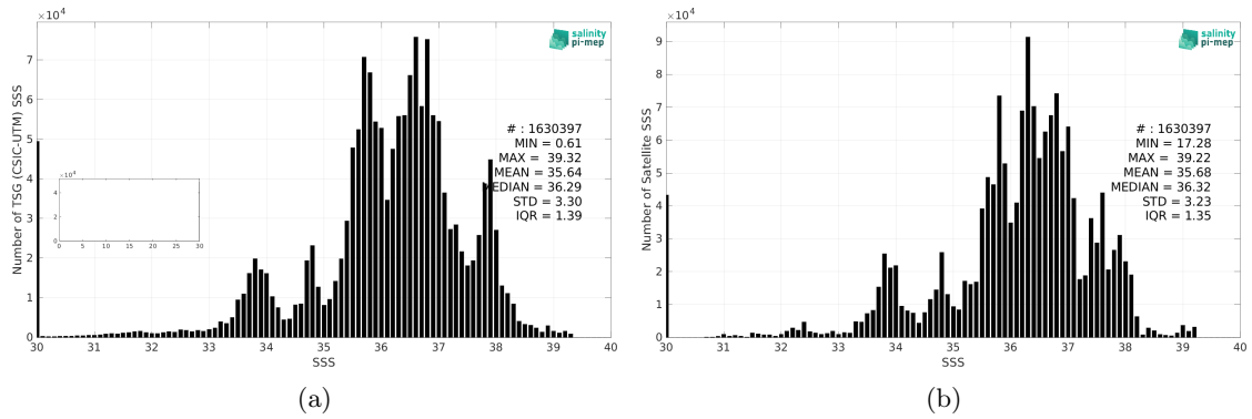
Figure 2: Histograms of SSS from TSG (CSIC-UTM) (a) and SMOS SSS L4 v1 - Weekly (CMEMS-CNR) (b) considering all match-up pairs per bins of 0.1 over the SMOS coastal zone (<800km) 60N-60S Pi-MEP region and for the full satellite product period.
