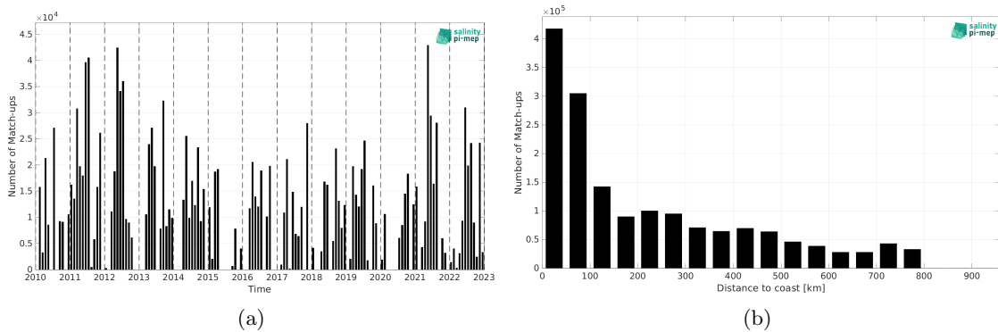
Figure 1: Number of match-ups between TSG (CSIC-UTM) and SMOS SSS L4 v1 - Weekly (CMEMS-CNR) SSS as a function of time (a) and as function of the distance to coast (b) over the SMOS coastal zone (<800km) 60N-60S Pi-MEP region and for the full satellite product period.
