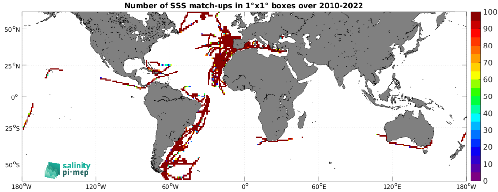
Figure 4: Number of SSS match-ups between TSG (CSIC-UTM) SSS and the SMOS SSS L4 v1 - Weekly (CMEMS-CNR) SSS product for the SMOS coastal zone (<800km) 60N-60S Pi-MEP region over 1^{\circ} \times 1^{\circ} boxes and for the full satellite product period.
