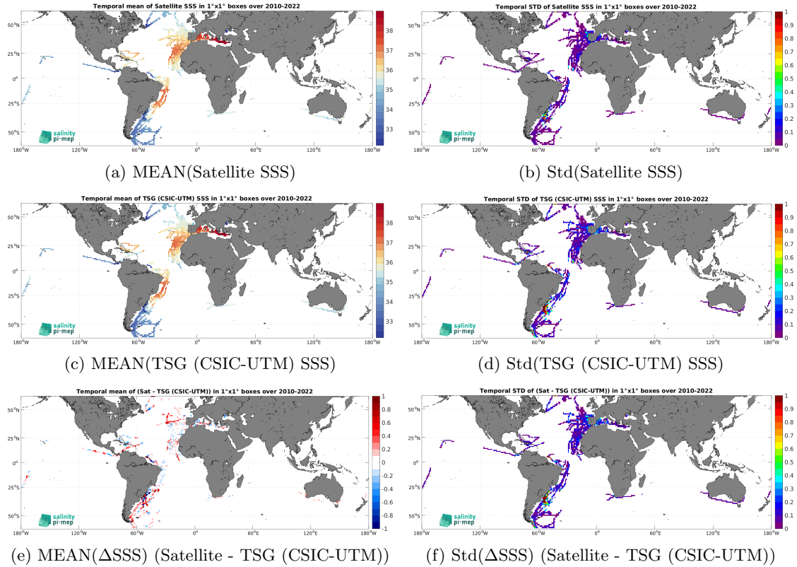
Figure 6: Temporal mean (left) and Std (right) of SSS from SMOS SSS L4 v1 - Weekly (CMEMS-CNR) (top), TSG (CSIC-UTM) (middle), and of \Delta SSS (Satellite - TSG (CSIC-UTM)). Only match-up pairs are used to generate these maps.
