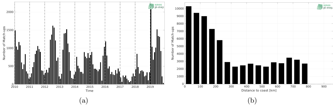
Figure 1: Number of match-ups between Marine mammals and SMOS SSS L4 v1 - Weekly (CMEMS-CNR) SSS as a function of time (a) and as function of the distance to coast (b) over the SMOS coastal zone (<800km) 60N-60S Pi-MEP region and for the full satellite product period.
