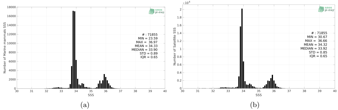
Figure 2: Histograms of SSS from Marine mammals (a) and SMOS SSS L4 v1 - Weekly (CMEMS-CNR) (b) considering all match-up pairs per bins of 0.1 over the SMOS coastal zone (<800km) 60N-60S Pi-MEP region and for the full satellite product period.
