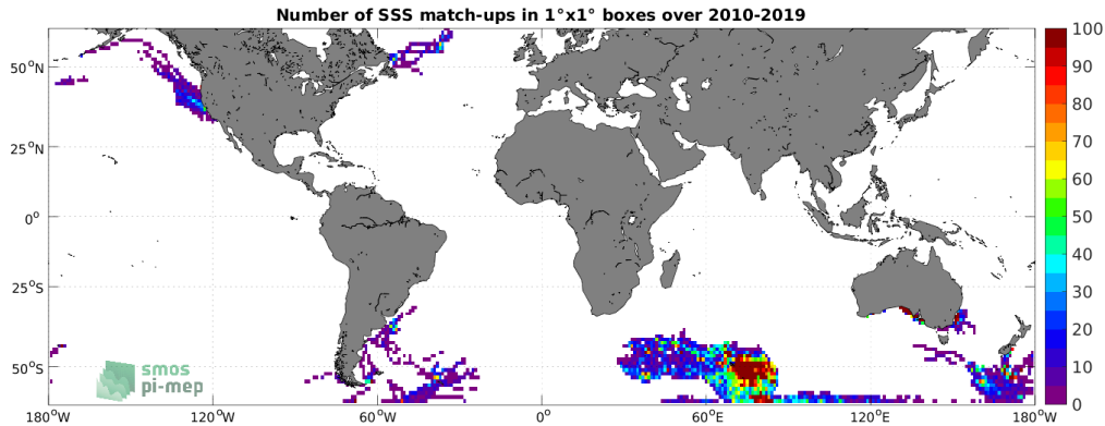
Figure 4: Number of SSS match-ups between Marine mammals SSS and the SMOS SSS L4 v1 - Weekly (CMEMS-CNR) SSS product for the SMOS coastal zone (<800km) 60N-60S Pi-MEP region over 1^{\circ} \times 1^{\circ} boxes and for the full satellite product period.
