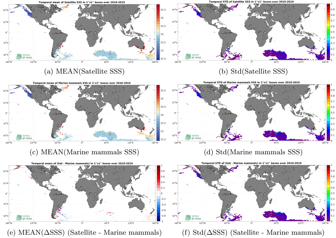
Figure 6: Temporal mean (left) and Std (right) of SSS from SMOS SSS L4 v1 - Weekly (CMEMS-CNR) (top), Marine mammals (middle), and of \Delta SSS (Satellite - Marine mammals). Only match-up pairs are used to generate these maps.
