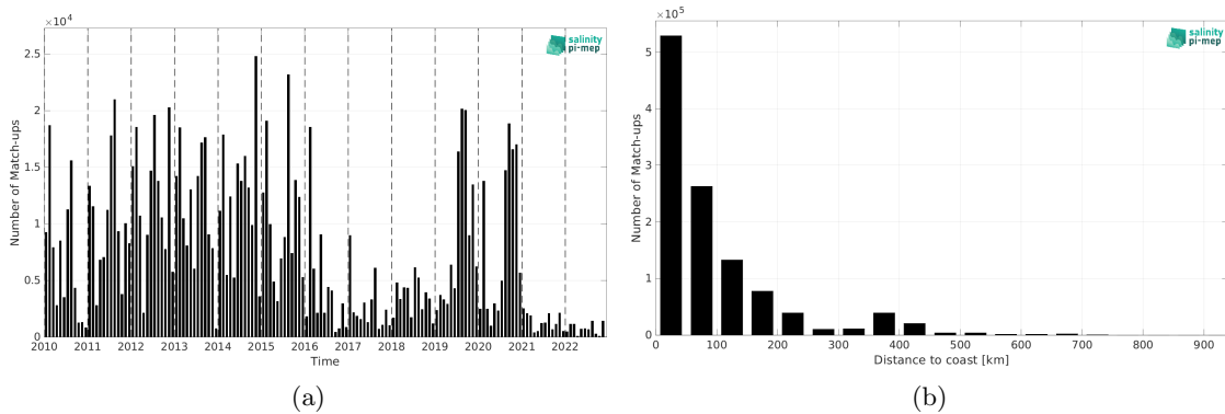
Figure 1: Number of match-ups between ICES and SMOS SSS L4 v1 - Weekly (CMEMS-CNR) SSS as a function of time (a) and as function of the distance to coast (b) over the SMOS coastal zone ( < 800\text{km} ) 60N-60S Pi-MEP region and for the full satellite product period.
